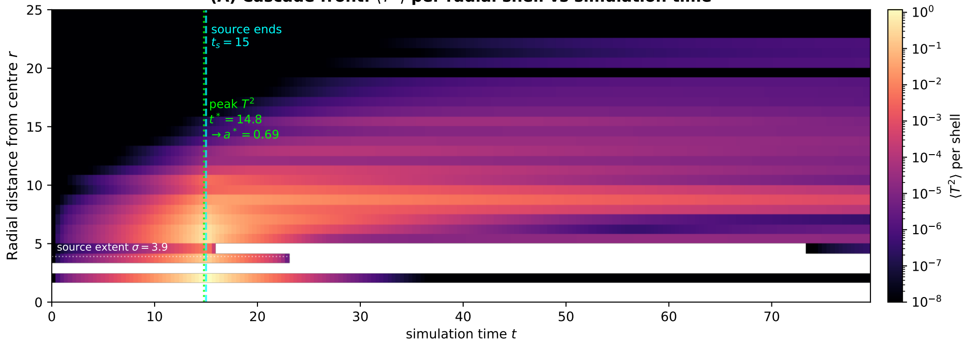
(A) Cascade front: \langle T^2 \rangle per radial shell vs simulation time
