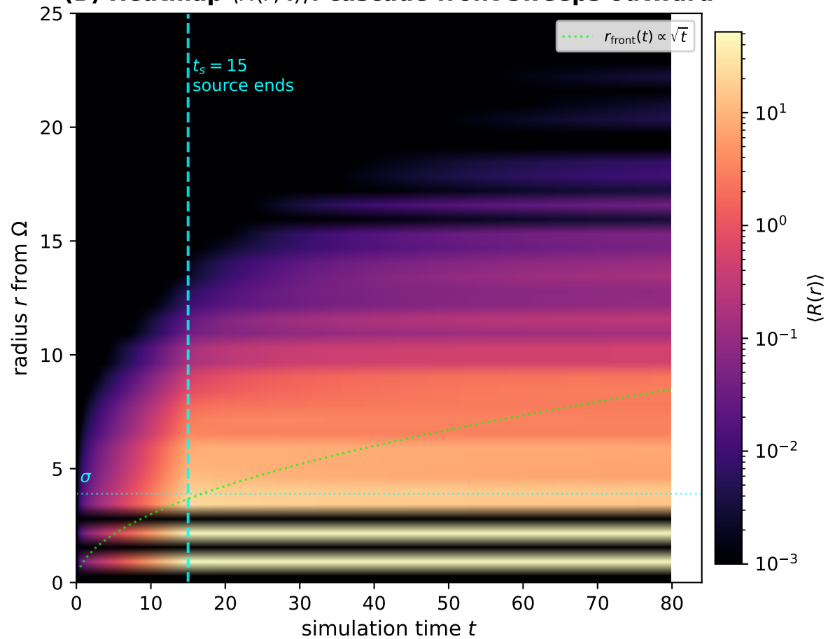
(B) Heatmap \langle R(r, t) \rangle : cascade front sweeps outward
