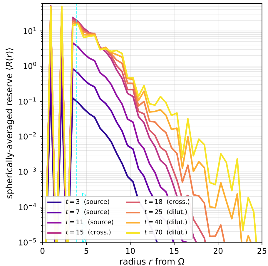
(A) Radial profile \langle R(r) \rangle at 8 snapshot times
