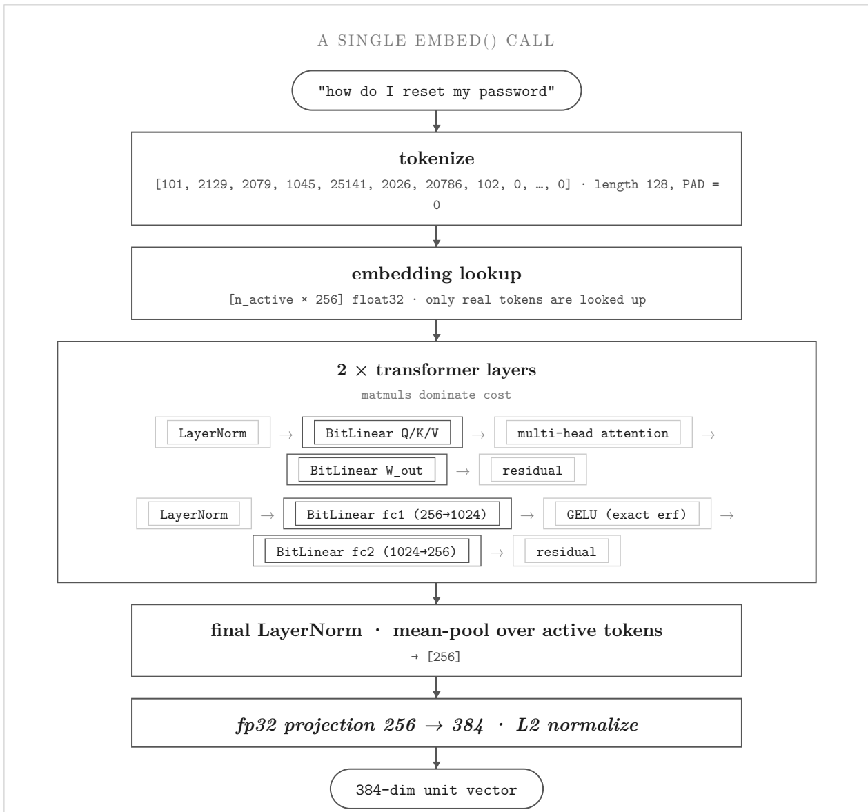
Figure 5. Execution trace of one embed() call, from raw text to the normalized 384-dim output vector.
