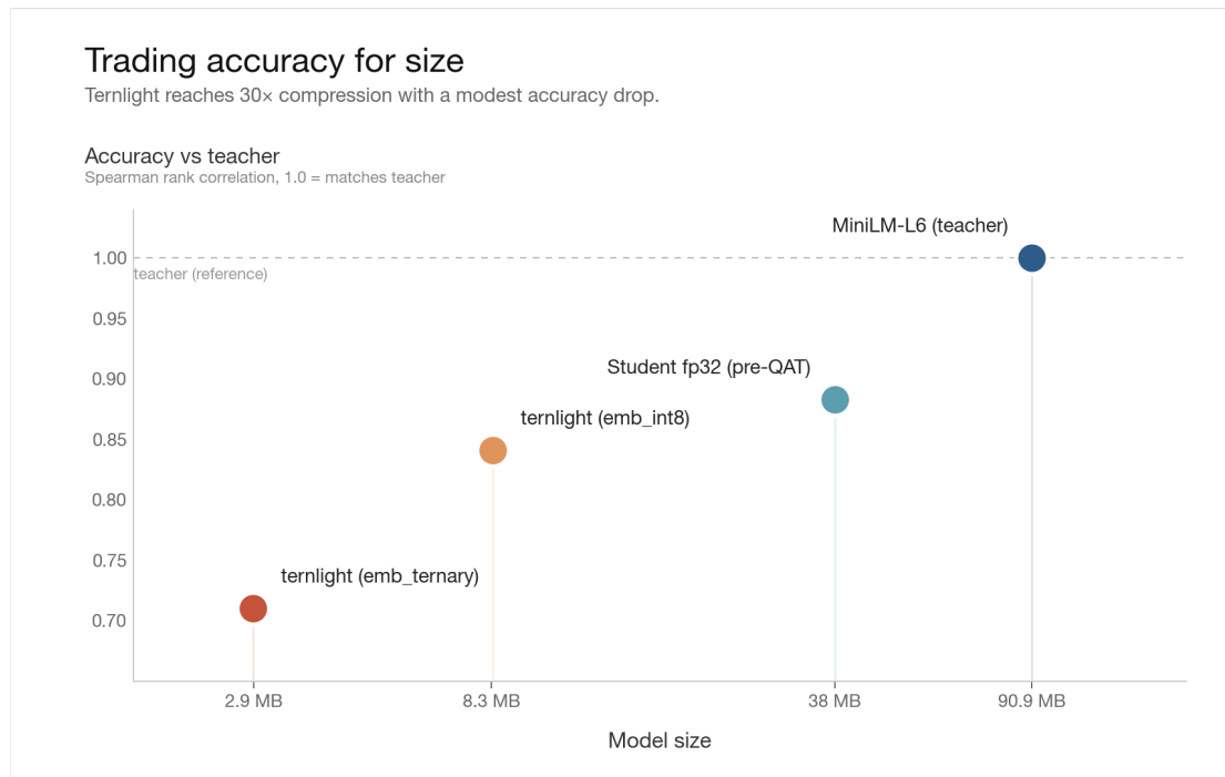
Figure 1. The size / accuracy trade-off. Teacher fidelity (Spearman vs MiniLM-L6) plotted against model size for the teacher, the fp32 student, and both ternlight ship variants. ternlight ( emb_ternary ) reaches ~30× compression for a modest fidelity drop.
