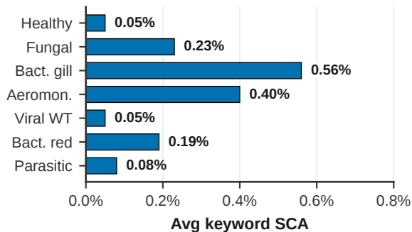
(a) Florence-2 keyword SCA
