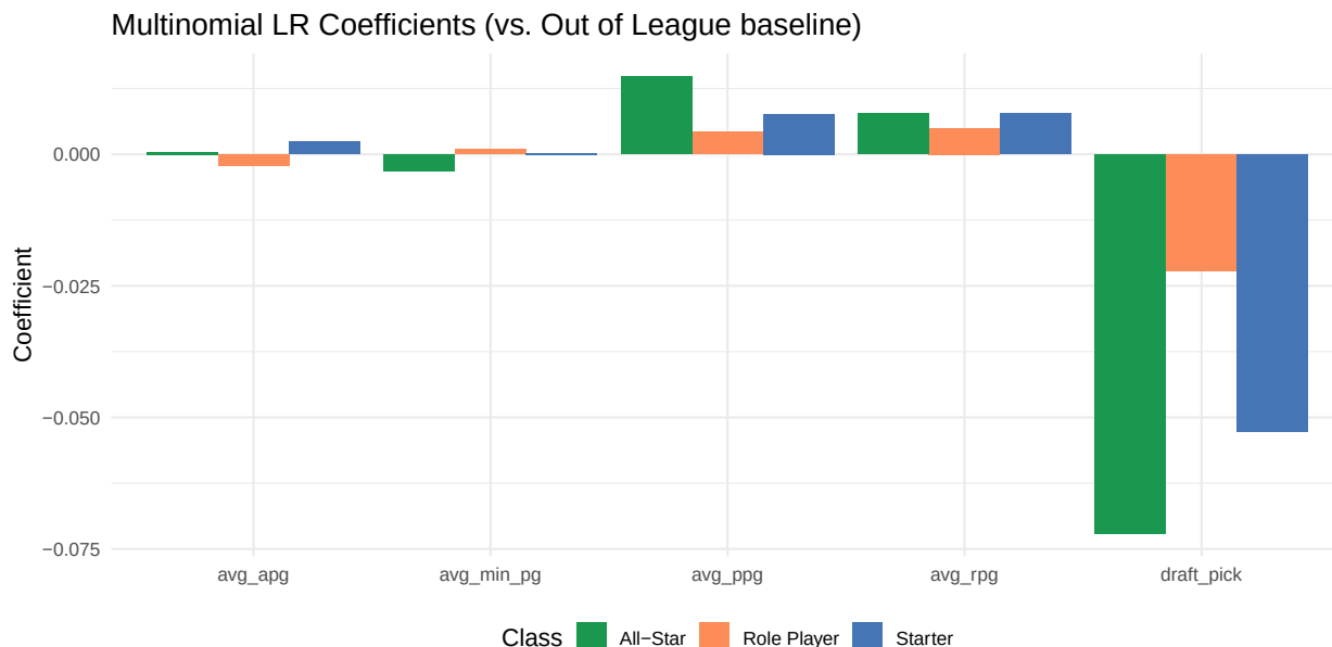
Figure 4: Multinomial logistic regression coefficients for key predictors, relative to Out of League baseline. Error bars omitted here; bootstrap CIs were computed for all coefficients.
