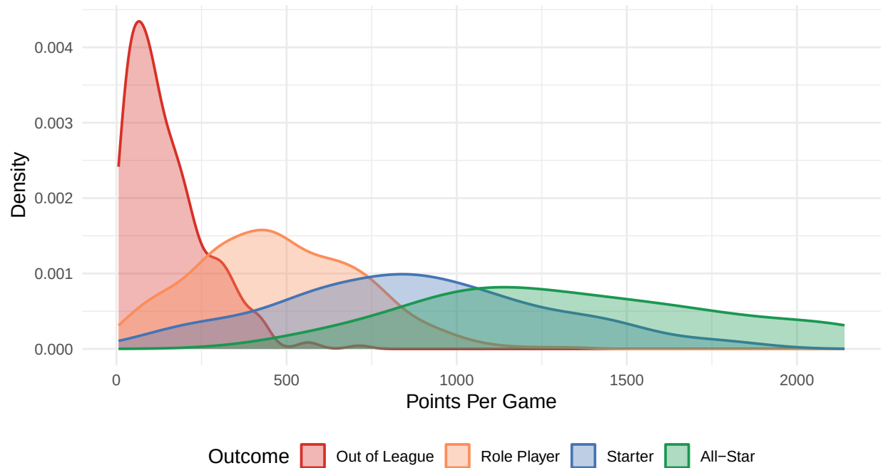
Figure 2: Distribution of average points per game in the first 1–3 seasons by career outcome tier. Better outcomes are associated with higher early scoring, though the distributions overlap considerably in the middle.
