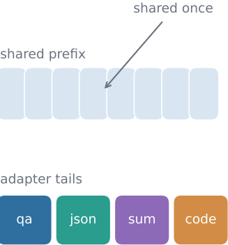
activated-style cache
