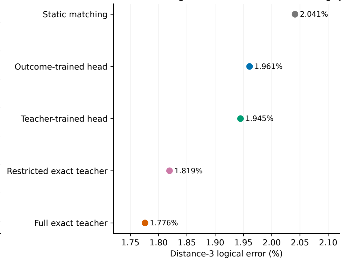
C The small grammar leaves most of the gap
