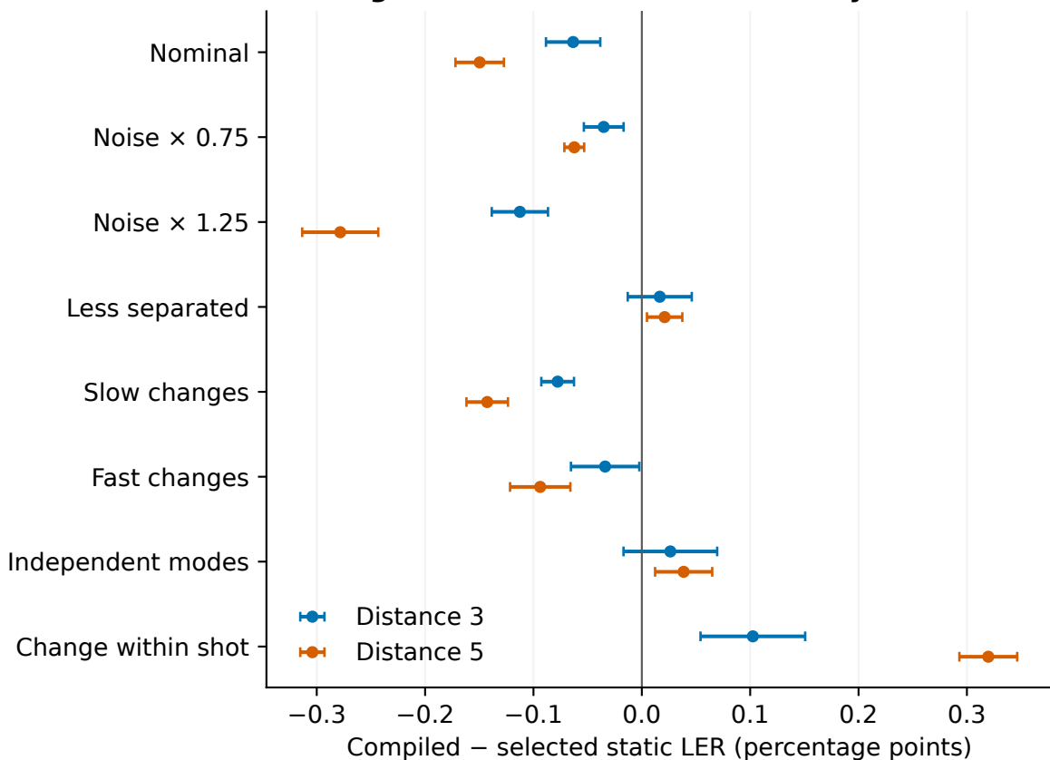
A The gain has a clear failure boundary
