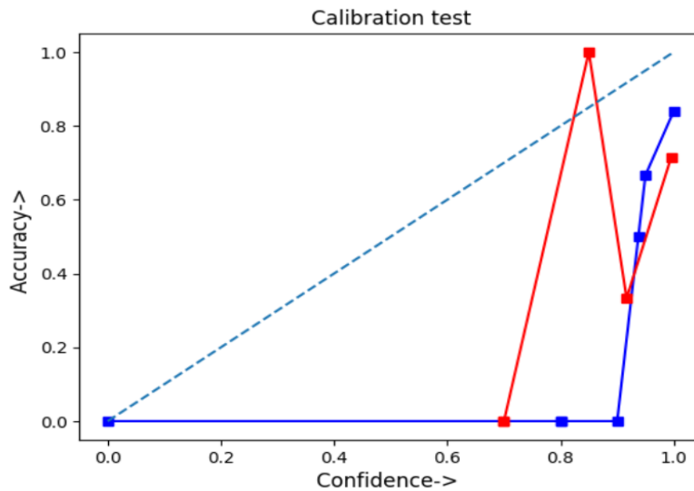
Figure 2. Reliability diagrams comparing predicted confidence and empirical accuracy across GPT-4o and Gemini 3.5.
