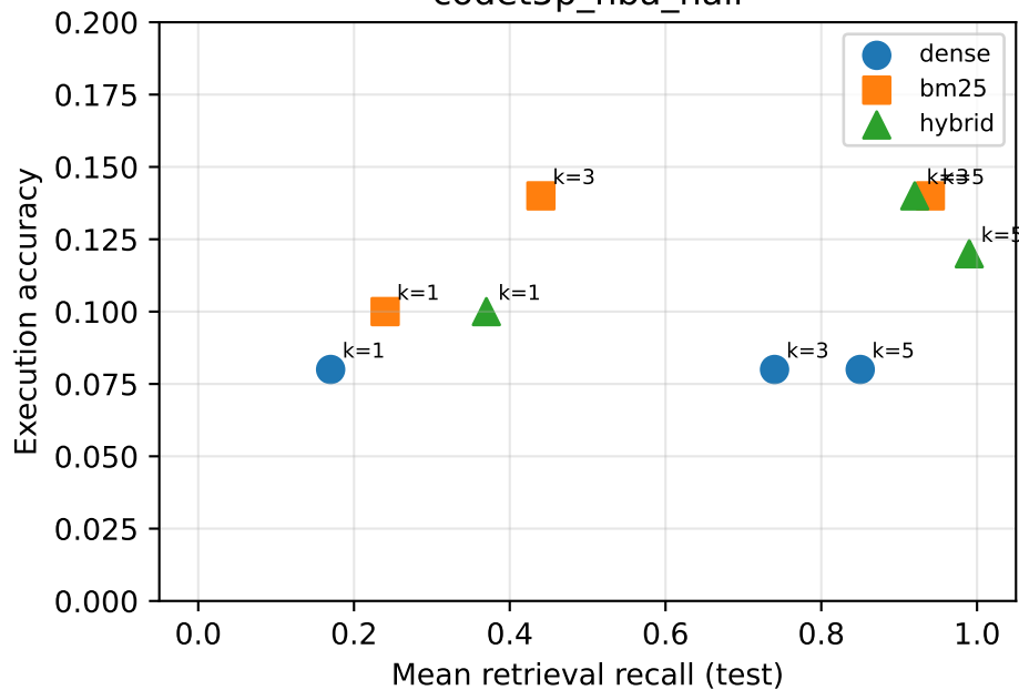
codet5p_nba_nall
