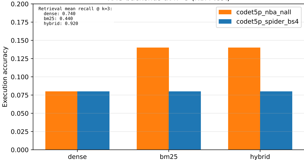
RAG backends at k=3 (NBA test)
