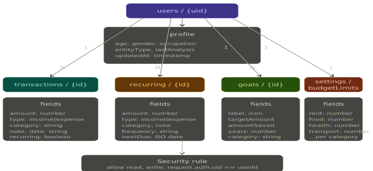
Figure 1: WealthWise Firestore Entity-Relationship Diagram
