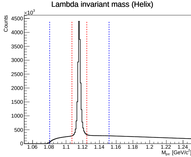
Figure 1: Invariant mass distribution of \Lambda . The sideband ranges are explicitly expanded to cover up to \pm 12\sigma .
