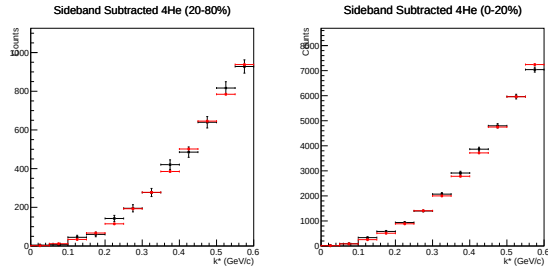
Figure 4: Step 3: Background-subtracted distributions ( True_{sig} - True_{SB} and Mix_{sig} - Mix_{SB} ).
