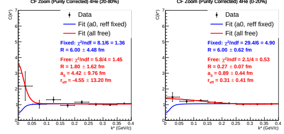
Figure 12: LL Fit on Purity-Corrected (CF-sub) CF.
