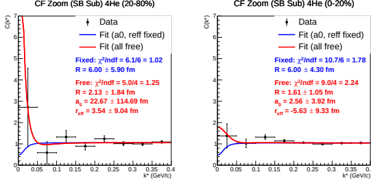
Figure 11: LL Fit on SB-Subtracted CF.
