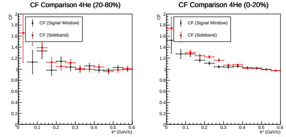
Figure 9: Step 4: Comparison of CF_{sig} and CF_{side} . The background CF is relatively flat compared to the signal.
