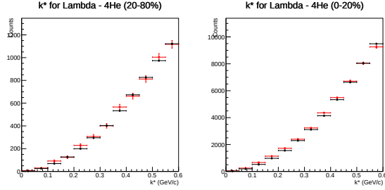
Figure 6: Step 1: Raw True and Mixed k^* distributions in the Signal Window.
