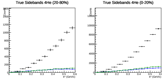
Figure 8: Step 3: True k^* distributions compared between Signal Window (black) and Sidebands (color).
