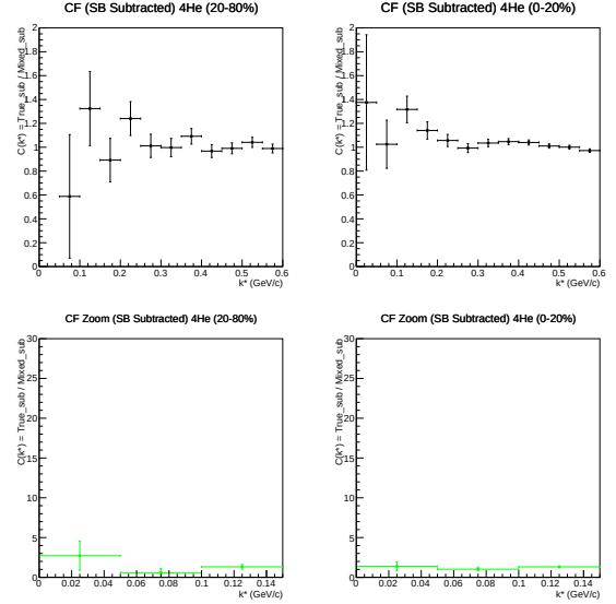
Figure 5: Step 4: Final SB-Subtracted CF, obtained by dividing the subtracted True by the subtracted Mixed distribution.
