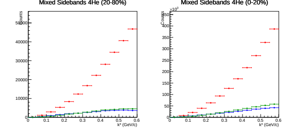
Figure 3: Step 2: Raw Mixed k^* distributions compared between Signal Window (red) and Sidebands (color).
