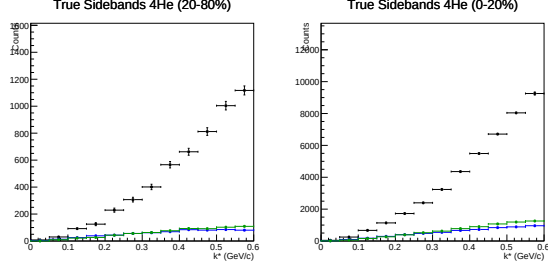
Figure 2: Step 1: Raw True k^* distributions compared between Signal Window (black) and Sidebands (color).
