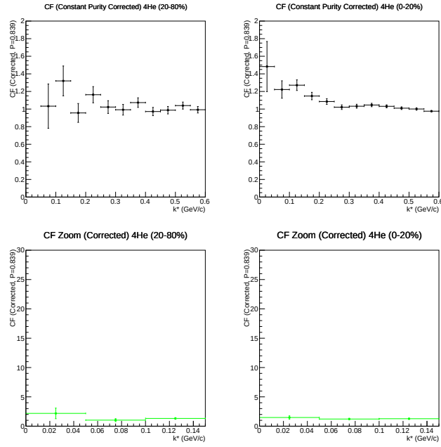
Figure 10: Step 5: Final Purity-Corrected CF. The background correlation ( CF_{SB} ) has been subtracted using the fixed purity ( P \approx 0.839 ).
