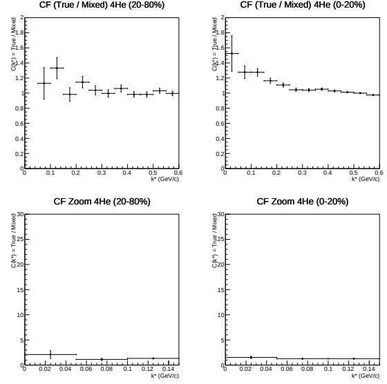
Figure 7: Step 2: CF_{sig} (True/Mixed) in the Signal Window.
