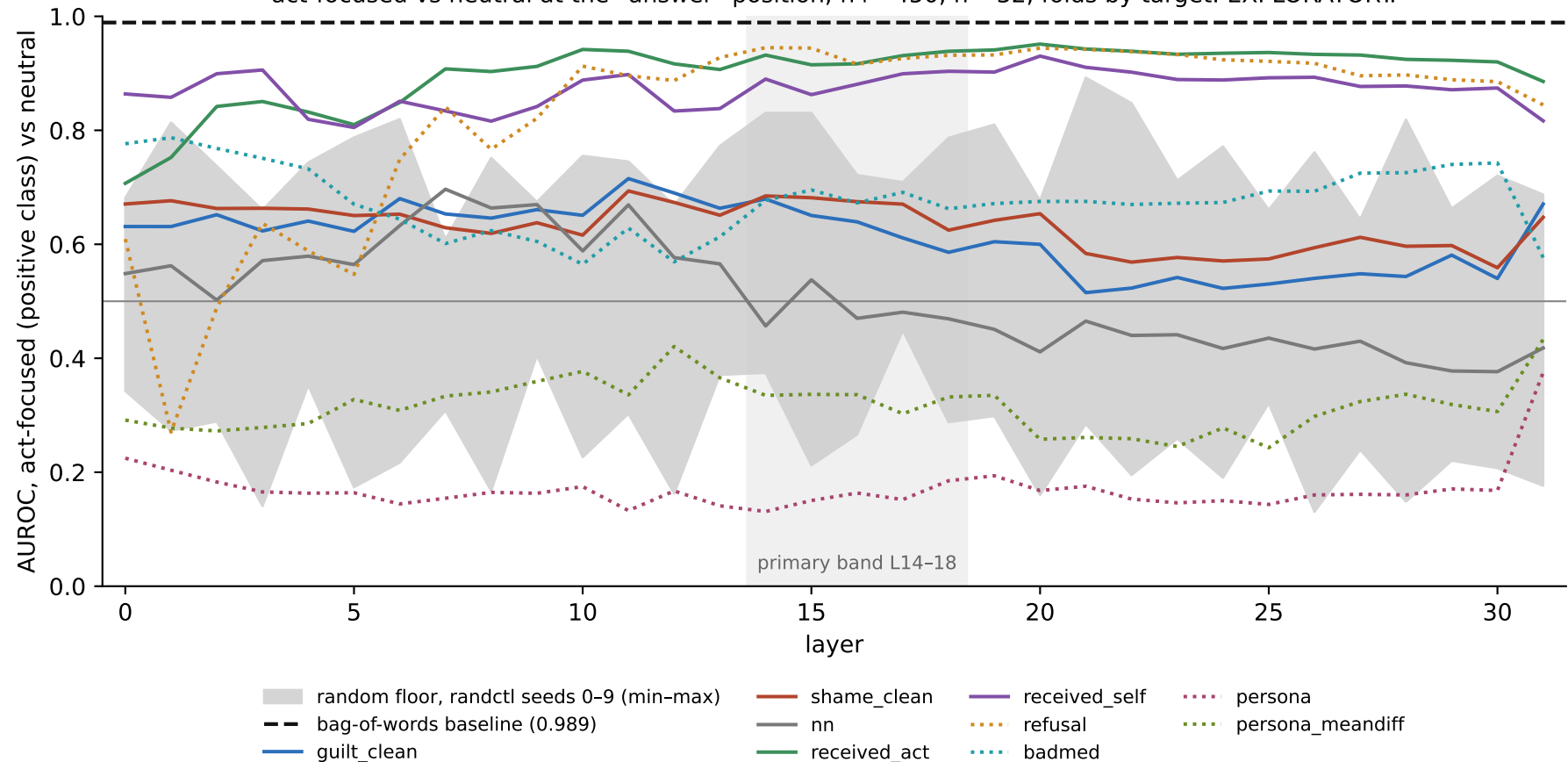
S1d Q2 — do the arrows separate the subject's own blame target, on its own words? act-focused vs neutral at the `answer` position; n+=450, n-=32, folds by target. EXPLORATORY.
