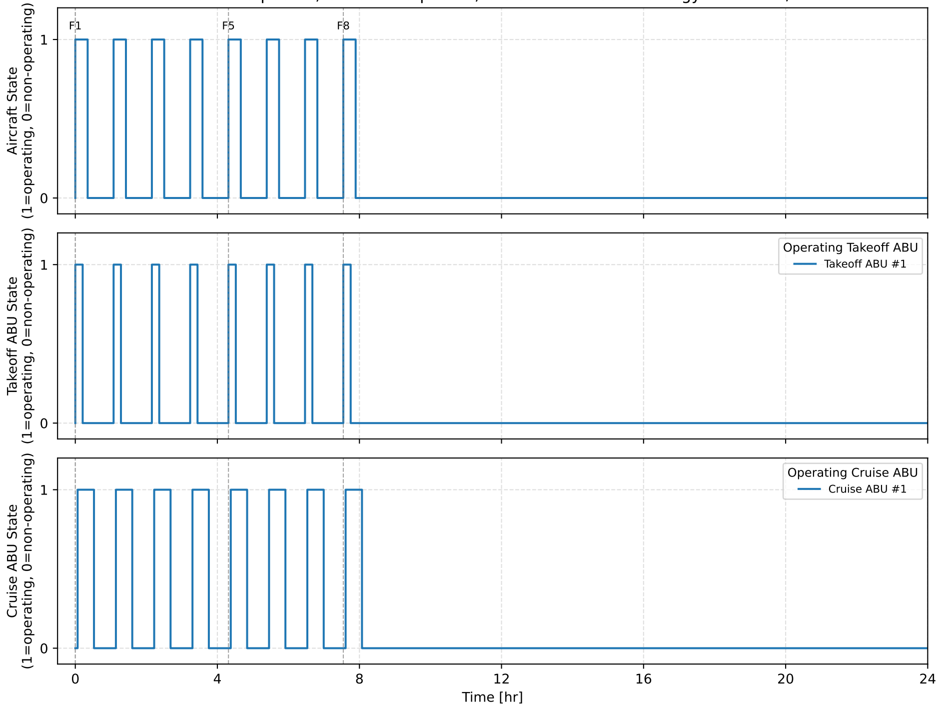
Daily Operational Timeline Takeoff ABU pool: 1, Cruise ABU pool: 1, Cruise ABU mission energy: 25.0 kWh/ABU
