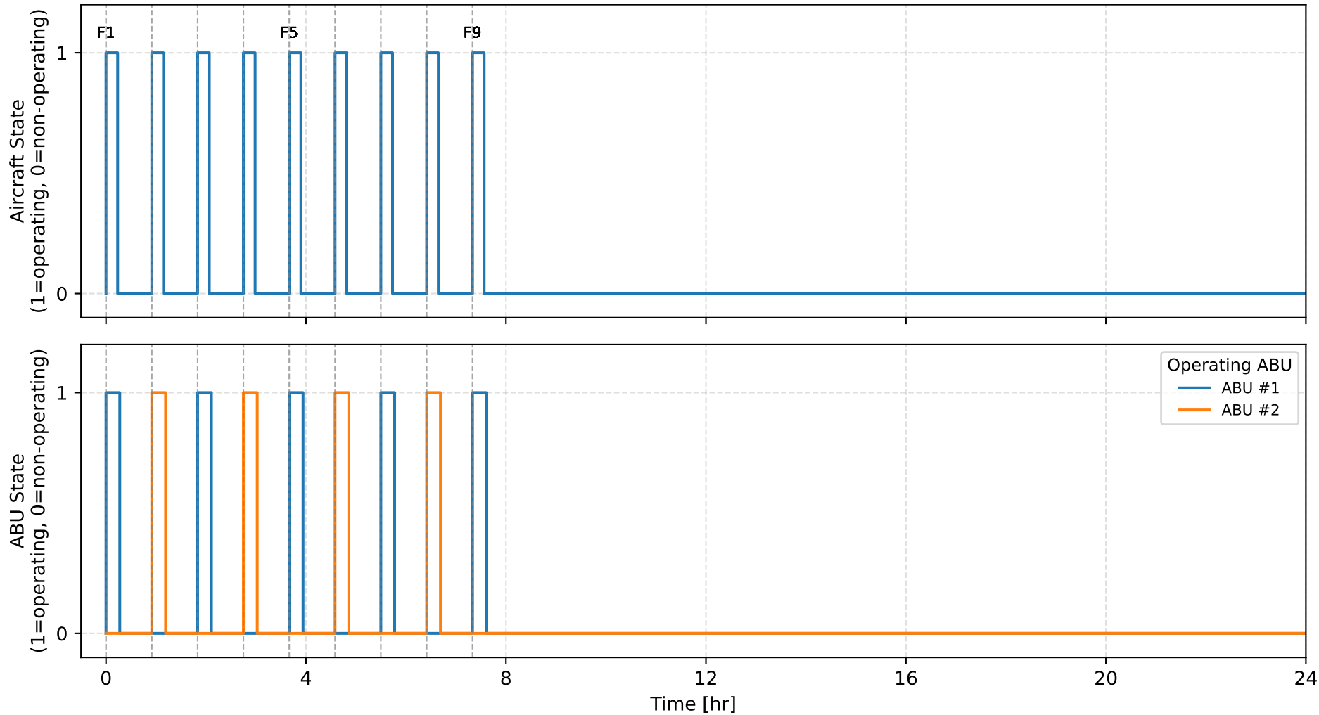
Daily Operational Timeline Number of ABUs: 2, ABU mission-energy: 50.0 kWh/ABU
