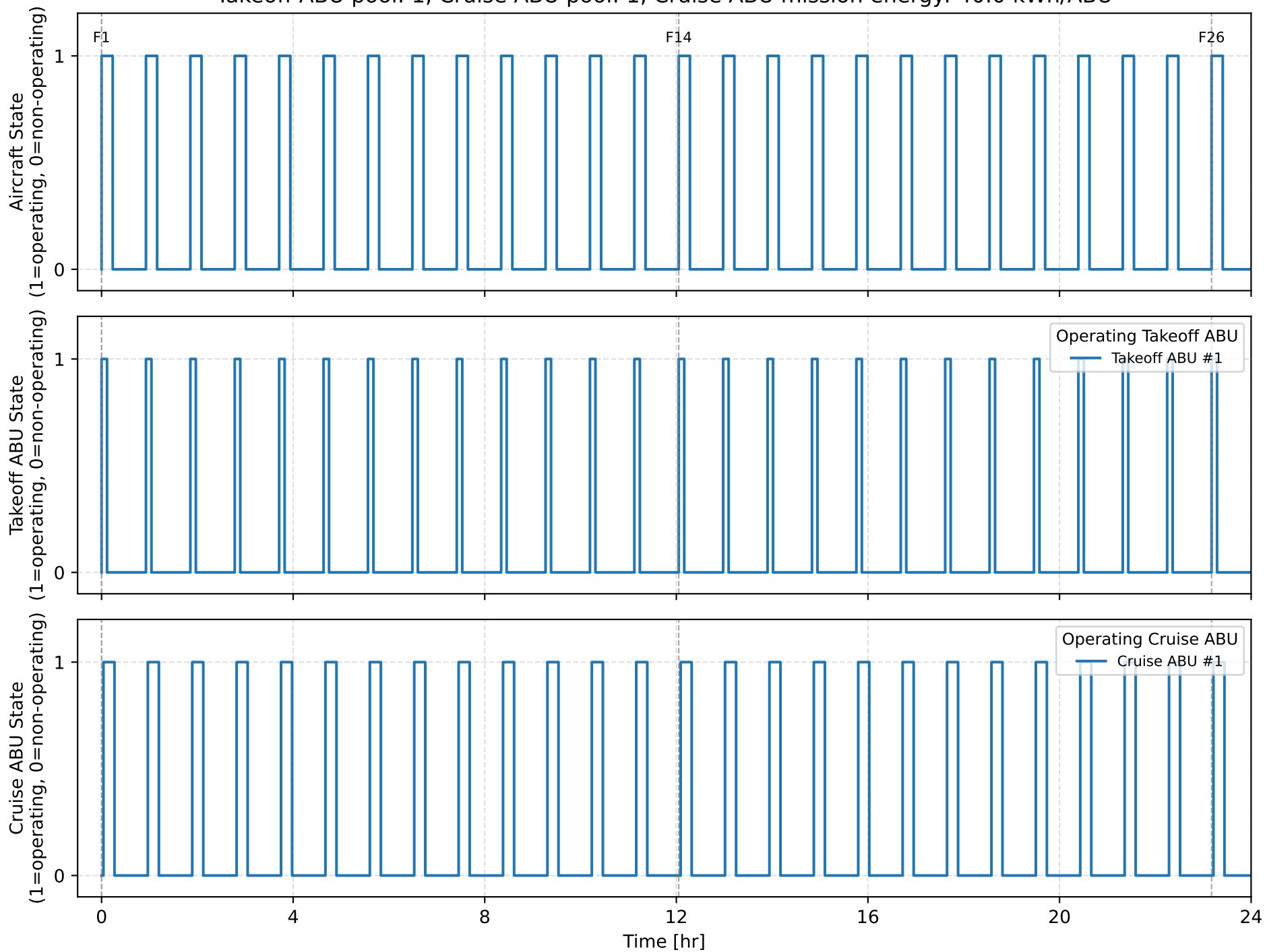
Daily Operational Timeline Takeoff ABU pool: 1, Cruise ABU pool: 1, Cruise ABU mission energy: 40.0 kWh/ABU
