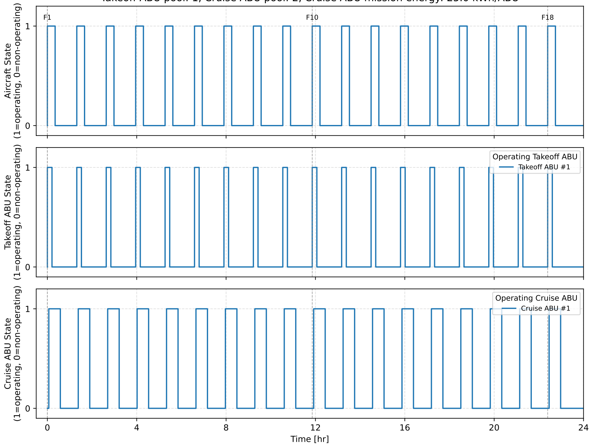
Daily Operational Timeline Takeoff ABU pool: 1, Cruise ABU pool: 2, Cruise ABU mission energy: 25.0 kWh/ABU
