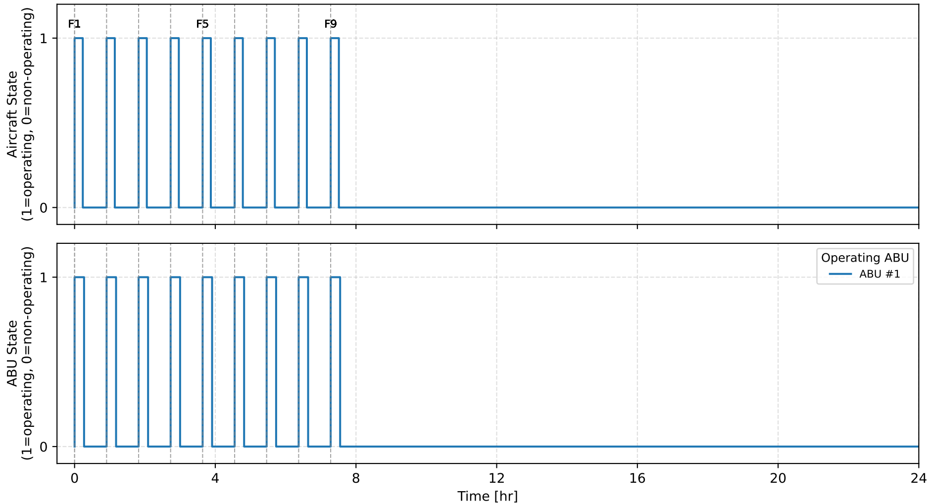
Daily Operational Timeline Number of ABUs: 1, ABU mission-energy: 35.0 kWh/ABU
