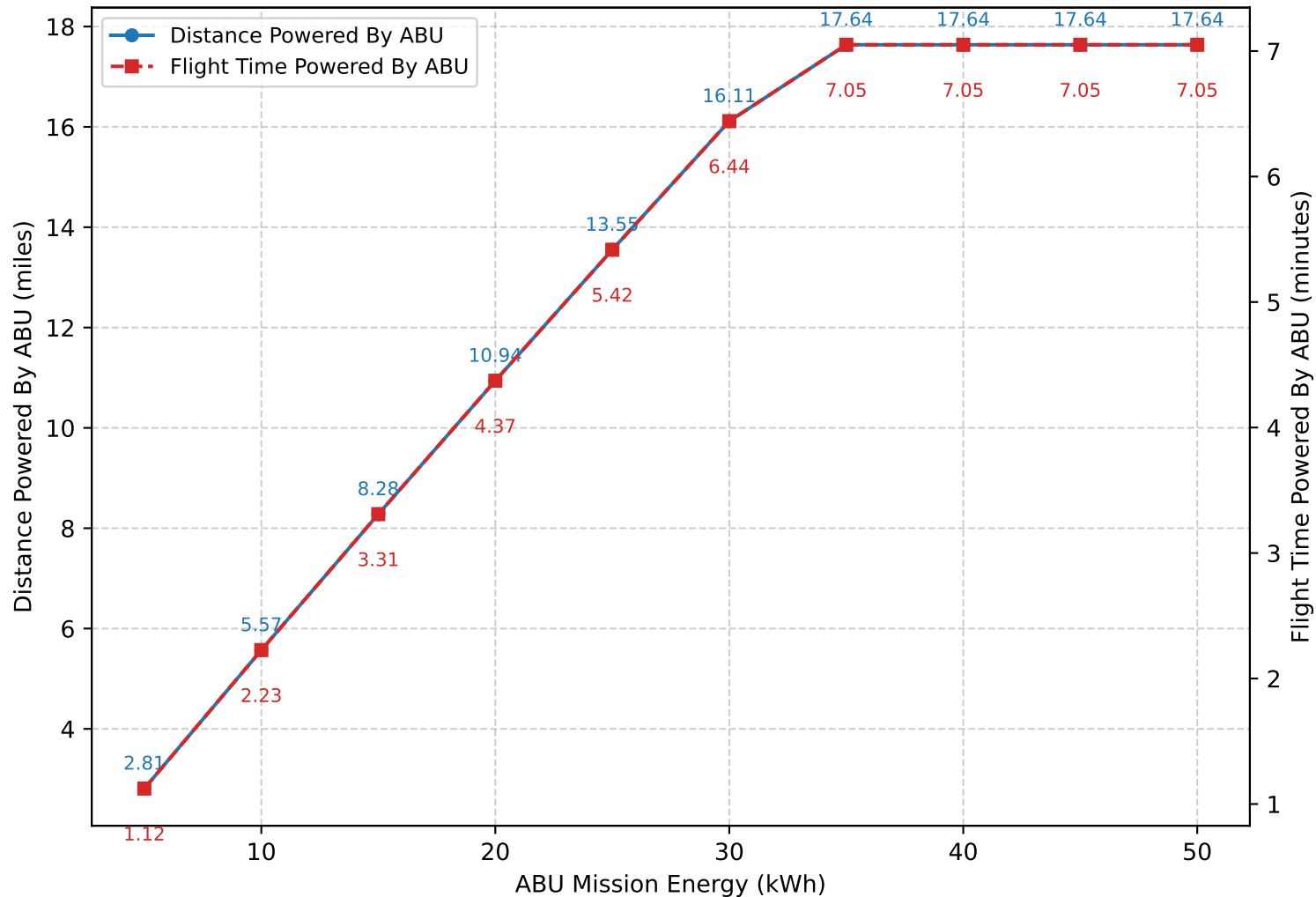
Flight Time And Distance Powered By ABU vs. ABU Mission Energy Detach On Depletion Or End Of Mission Segment
