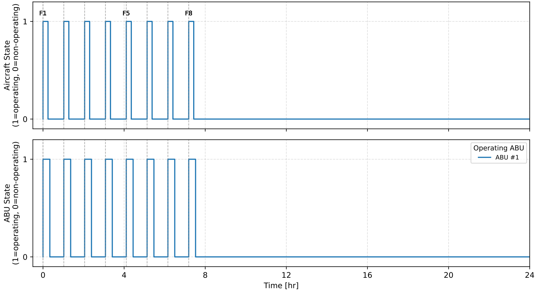
Daily Operational Timeline Number of ABUs: 1, ABU mission-energy: 30.0 kWh/ABU
