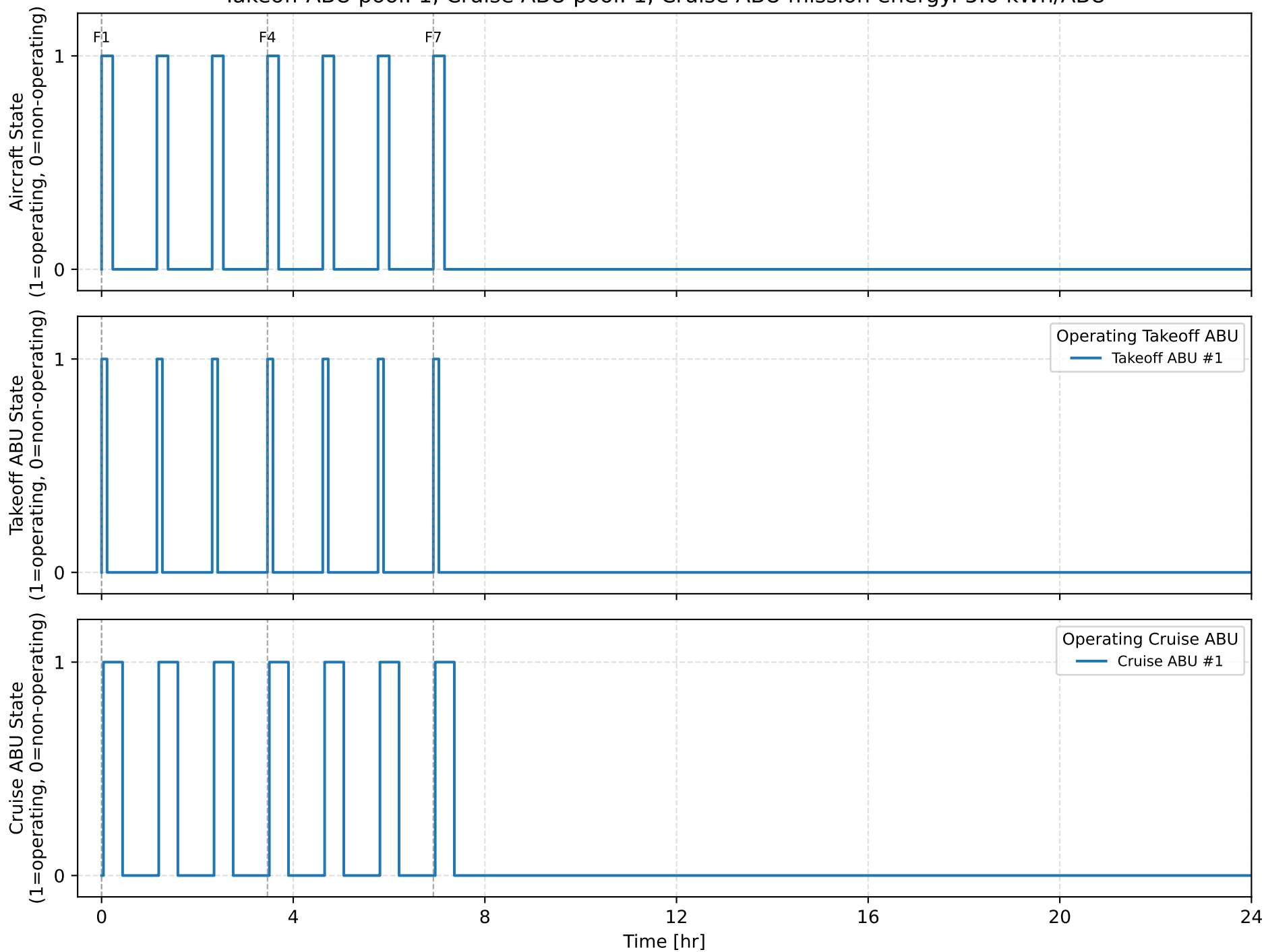
Daily Operational Timeline Takeoff ABU pool: 1, Cruise ABU pool: 1, Cruise ABU mission energy: 5.0 kWh/ABU
