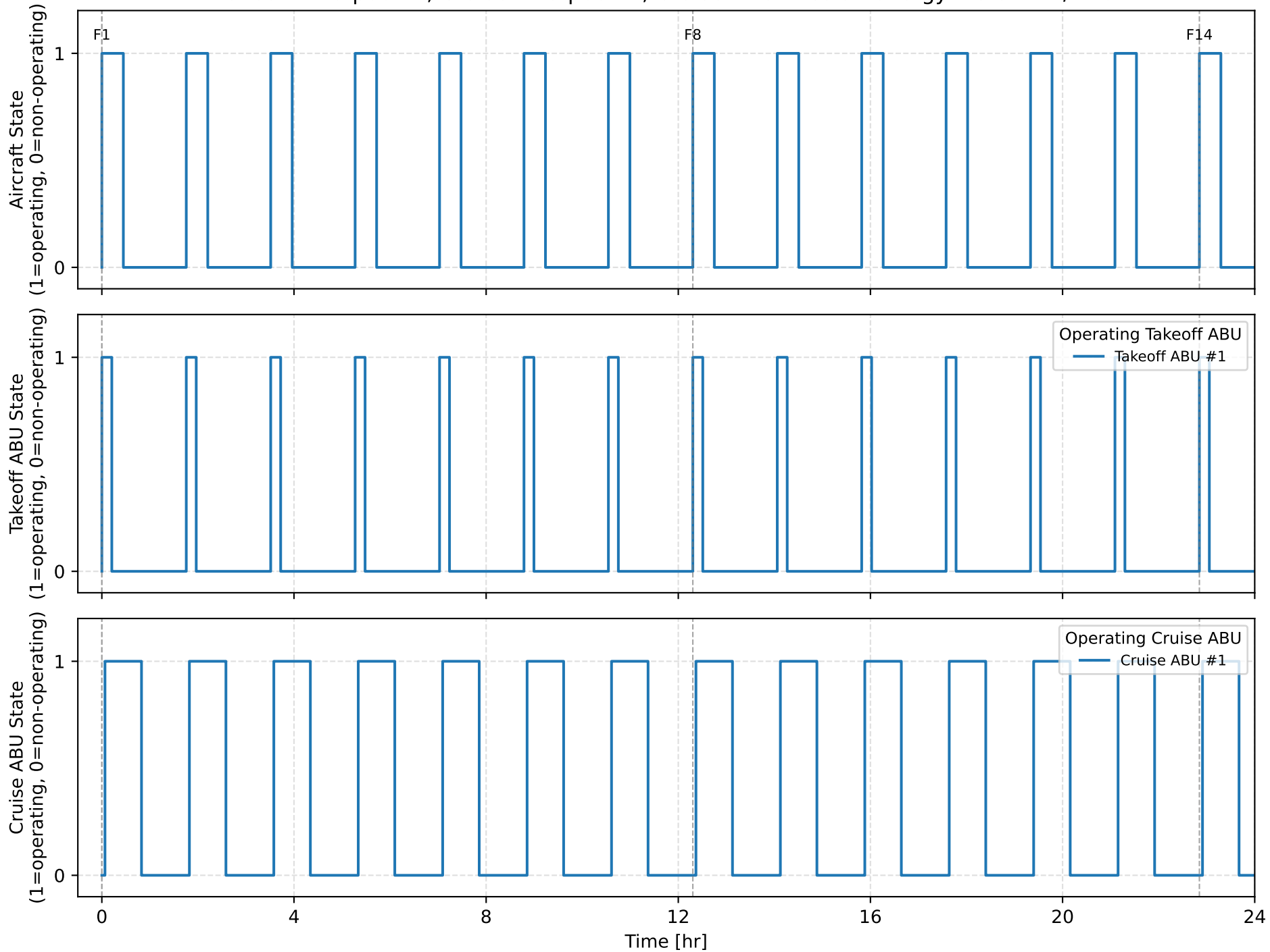
Daily Operational Timeline Takeoff ABU pool: 1, Cruise ABU pool: 2, Cruise ABU mission energy: 20.0 kWh/ABU
