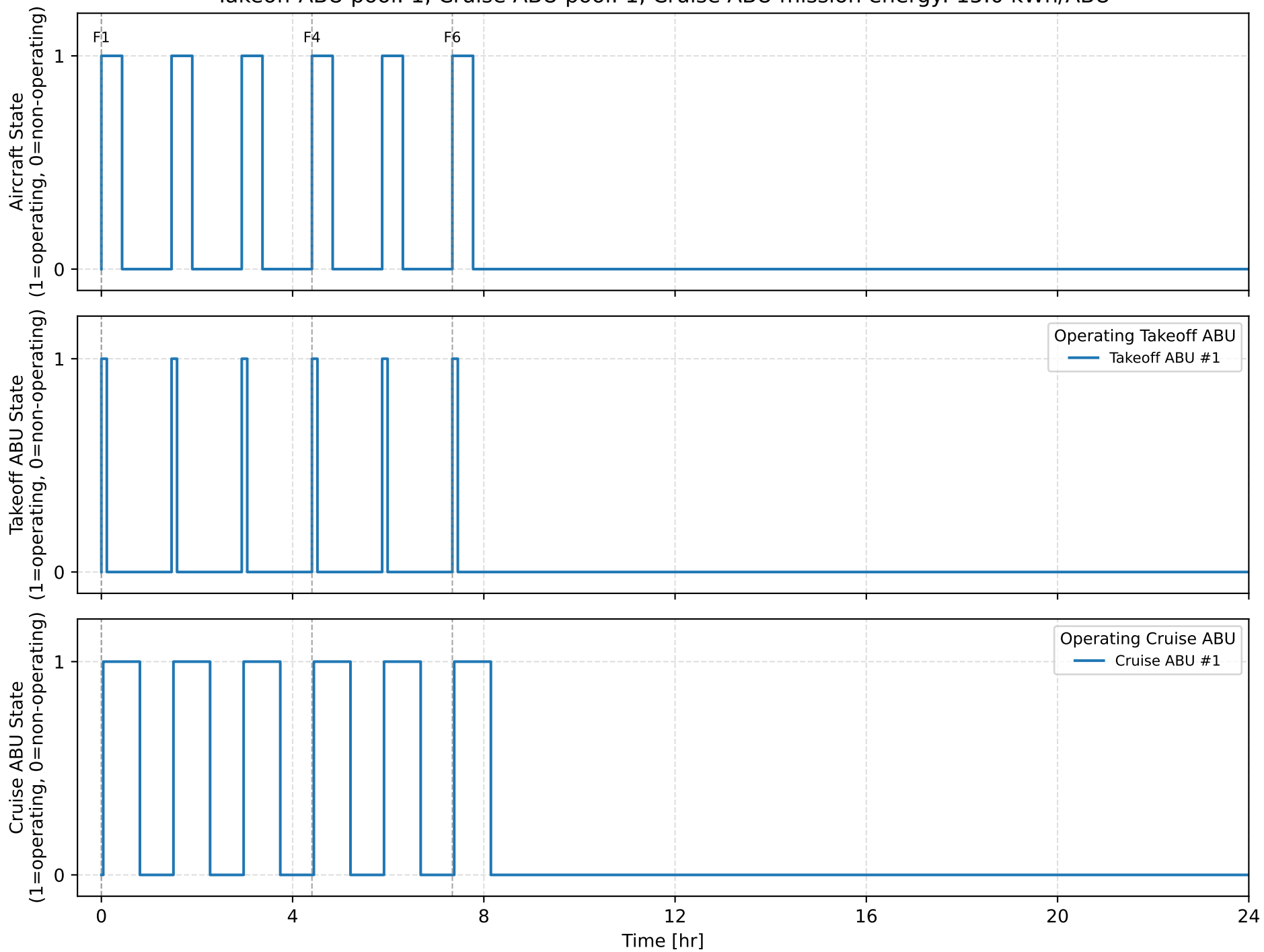
Daily Operational Timeline Takeoff ABU pool: 1, Cruise ABU pool: 1, Cruise ABU mission energy: 15.0 kWh/ABU
