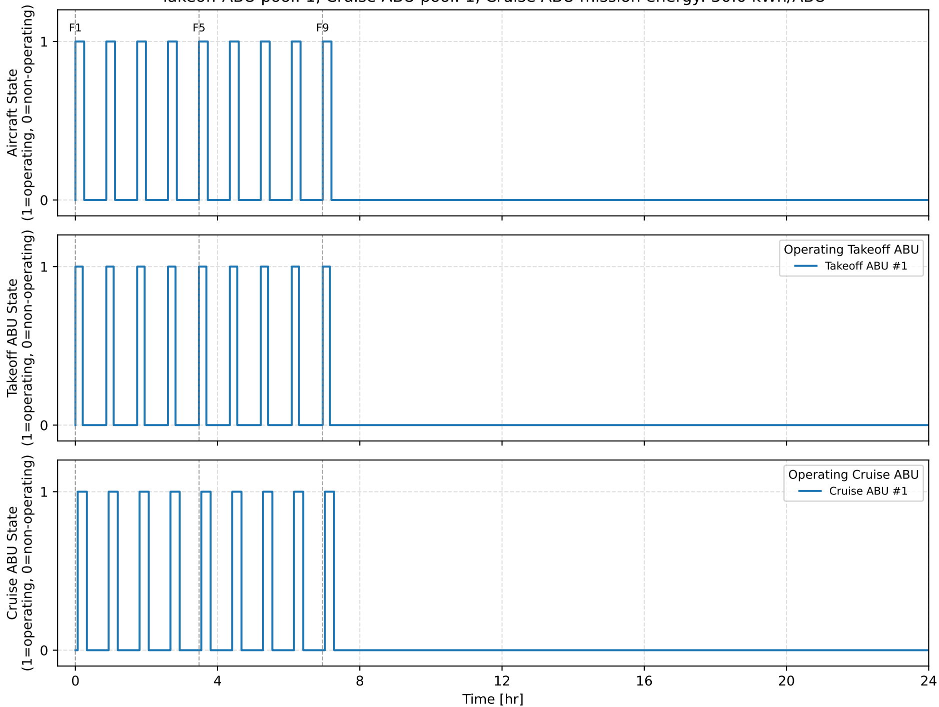
Daily Operational Timeline Takeoff ABU pool: 1, Cruise ABU pool: 1, Cruise ABU mission energy: 30.0 kWh/ABU
