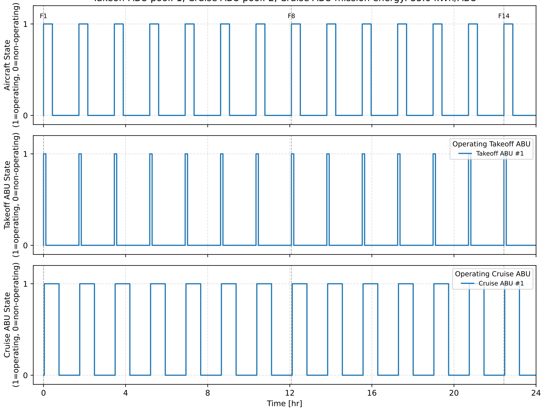
Daily Operational Timeline Takeoff ABU pool: 1, Cruise ABU pool: 2, Cruise ABU mission energy: 35.0 kWh/ABU
