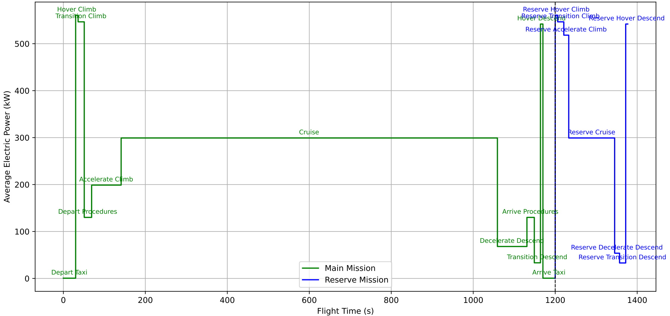
Power Profile
