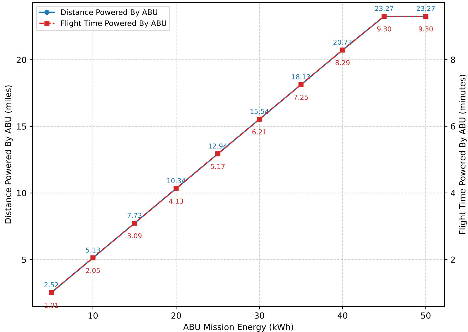
Flight Time And Distance Powered By ABU vs. ABU Mission Energy
