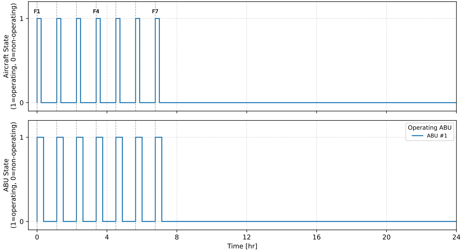
Daily Operational Timeline Number of ABUs: 2, ABU mission-energy: 20.0 kWh/ABU
