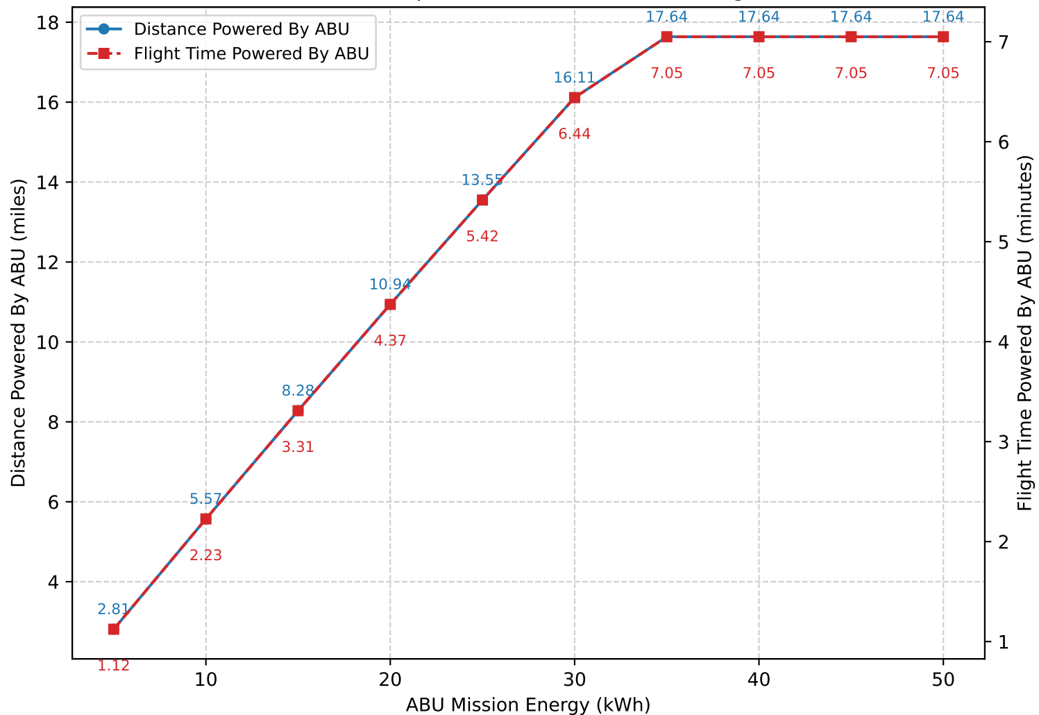
Flight Time And Distance Powered By ABU vs. ABU Mission Energy Detach On Depletion Or End Of Mission Segment
