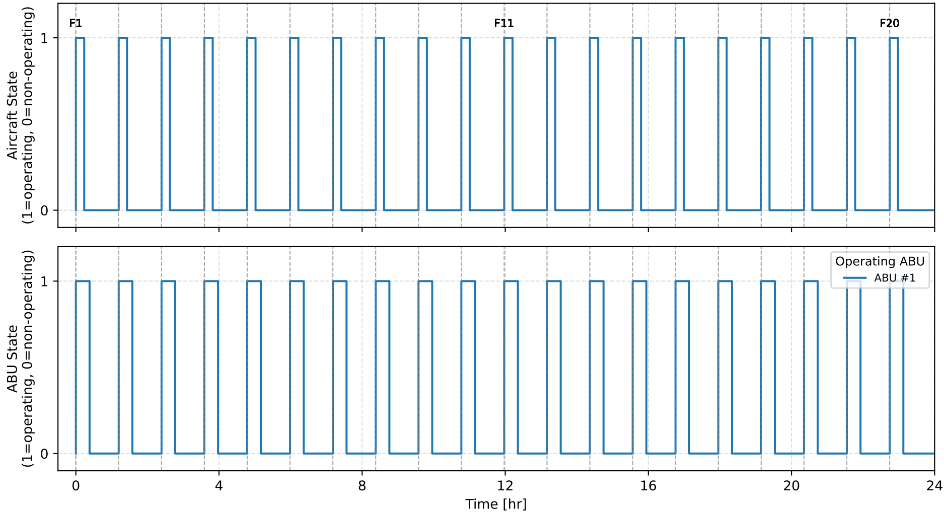
Daily Operational Timeline Number of ABUs: 1, ABU mission-energy: 20.0 kWh/ABU
