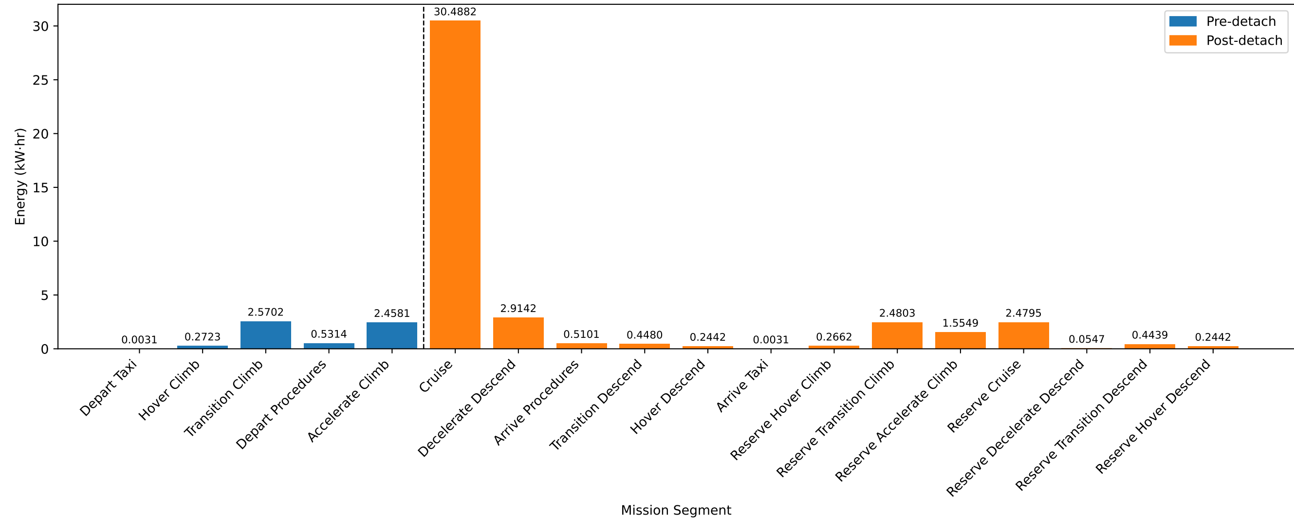
Mission Segment Energy - Detach After Accelerate Climb
