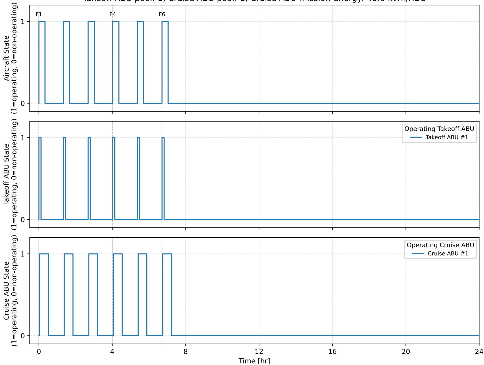
Daily Operational Timeline Takeoff ABU pool: 1, Cruise ABU pool: 1, Cruise ABU mission energy: 45.0 kWh/ABU
