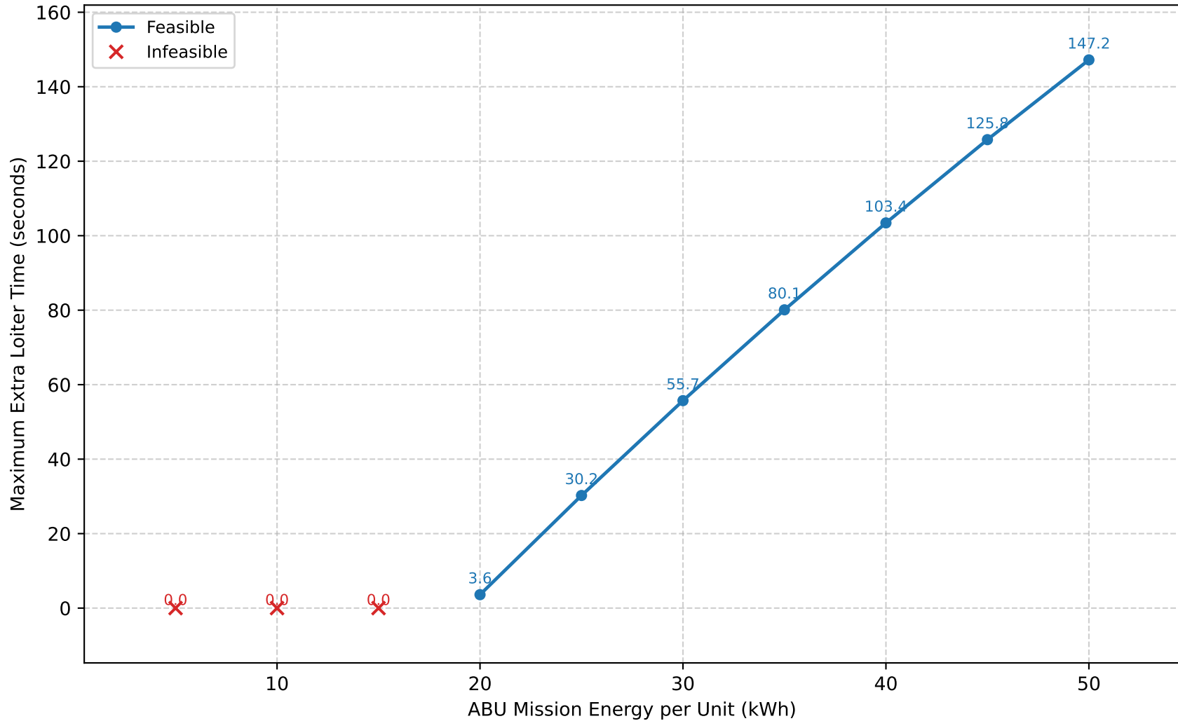
ABU Landing Safety Benefit Maximum Extra Loiter Time vs. ABU Mission Energy
