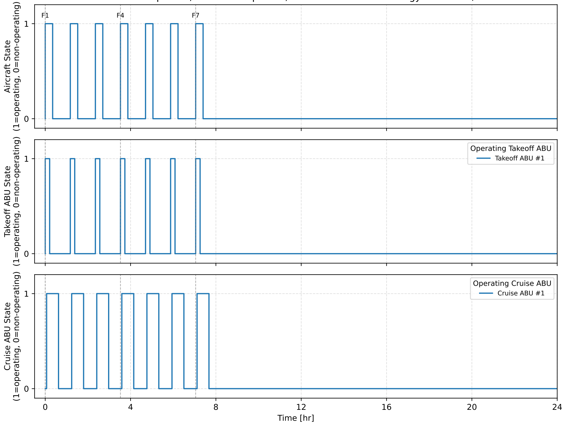
Daily Operational Timeline Takeoff ABU pool: 1, Cruise ABU pool: 2, Cruise ABU mission energy: 10.0 kWh/ABU
