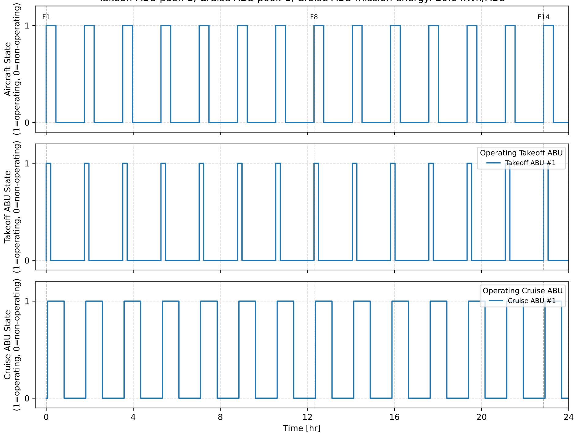
Daily Operational Timeline Takeoff ABU pool: 1, Cruise ABU pool: 1, Cruise ABU mission energy: 20.0 kWh/ABU
