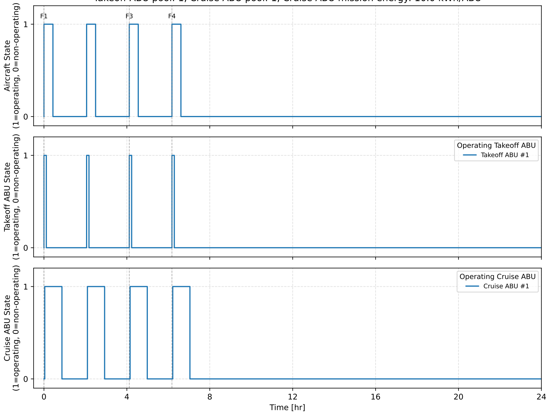
Daily Operational Timeline Takeoff ABU pool: 1, Cruise ABU pool: 1, Cruise ABU mission energy: 10.0 kWh/ABU
