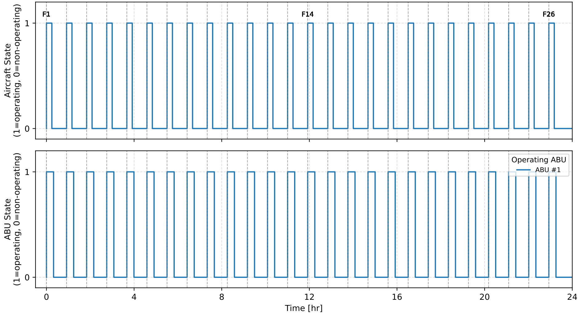
Daily Operational Timeline Number of ABUs: 2, ABU mission-energy: 35.0 kWh/ABU
