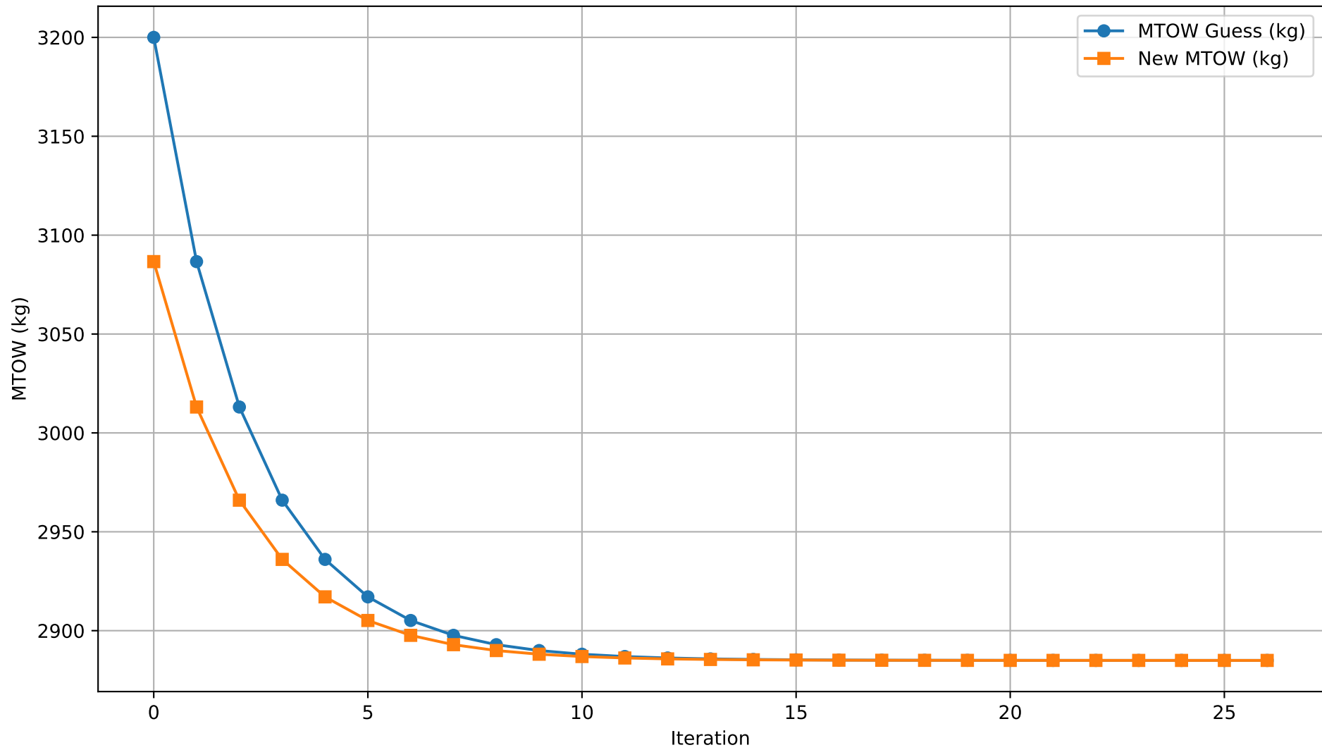
MTOW Iteration Convergence
