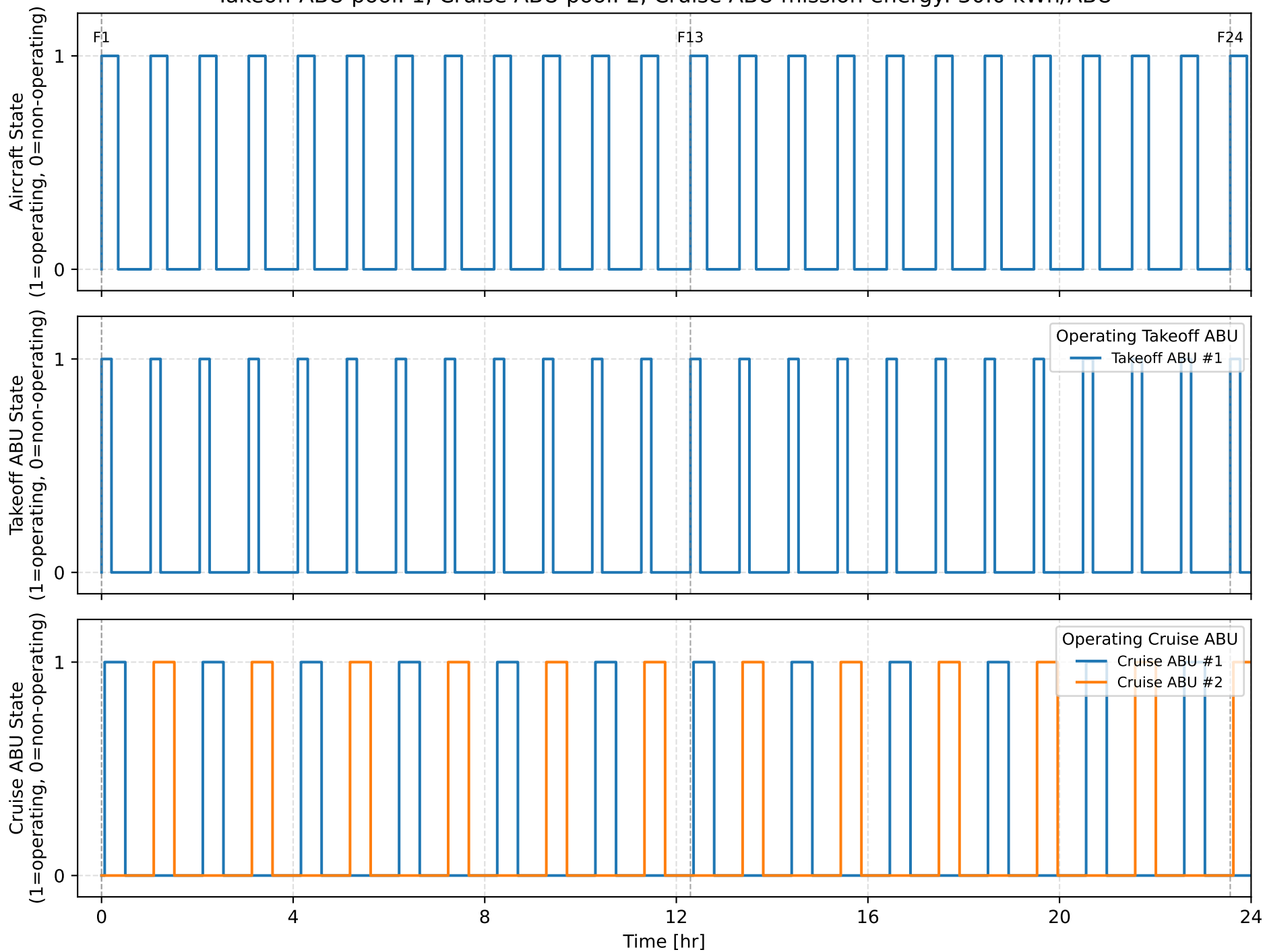
Daily Operational Timeline Takeoff ABU pool: 1, Cruise ABU pool: 2, Cruise ABU mission energy: 30.0 kWh/ABU
