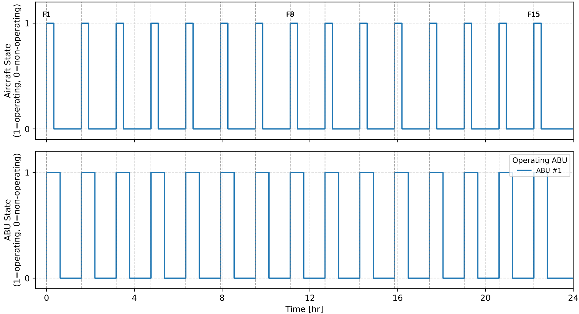
Daily Operational Timeline Number of ABUs: 2, ABU mission-energy: 15.0 kWh/ABU
