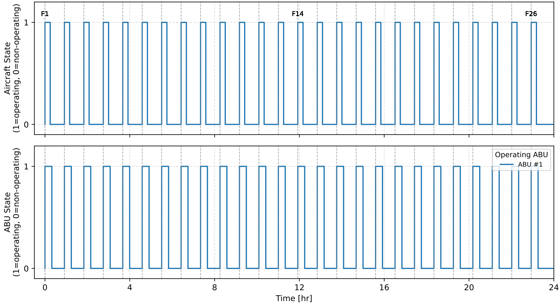
Daily Operational Timeline Number of ABUs: 2, ABU mission-energy: 30.0 kWh/ABU
