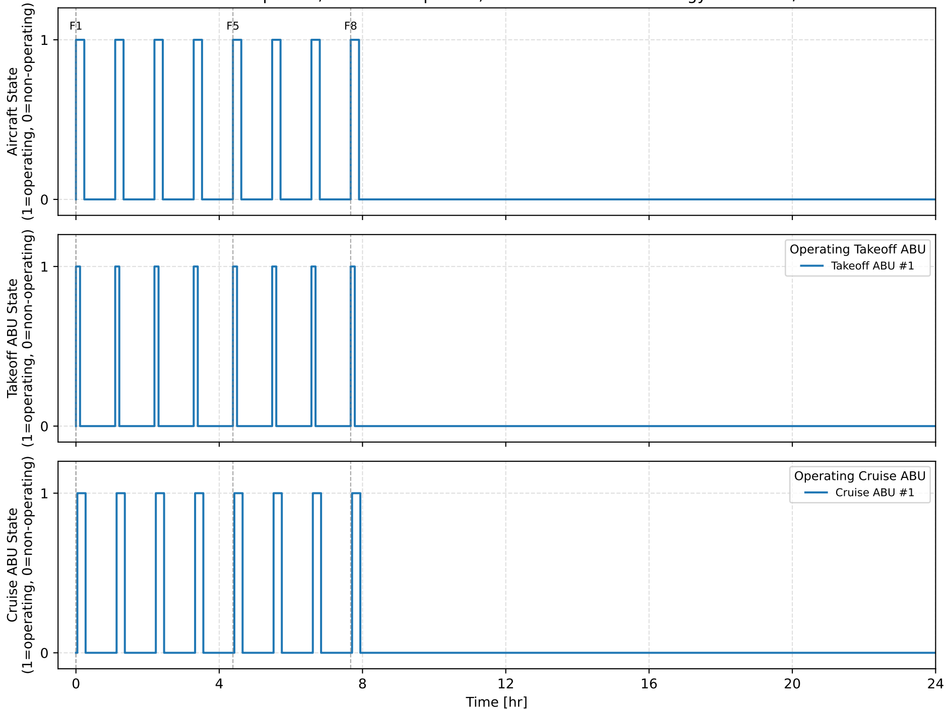
Daily Operational Timeline Takeoff ABU pool: 1, Cruise ABU pool: 1, Cruise ABU mission energy: 50.0 kWh/ABU
