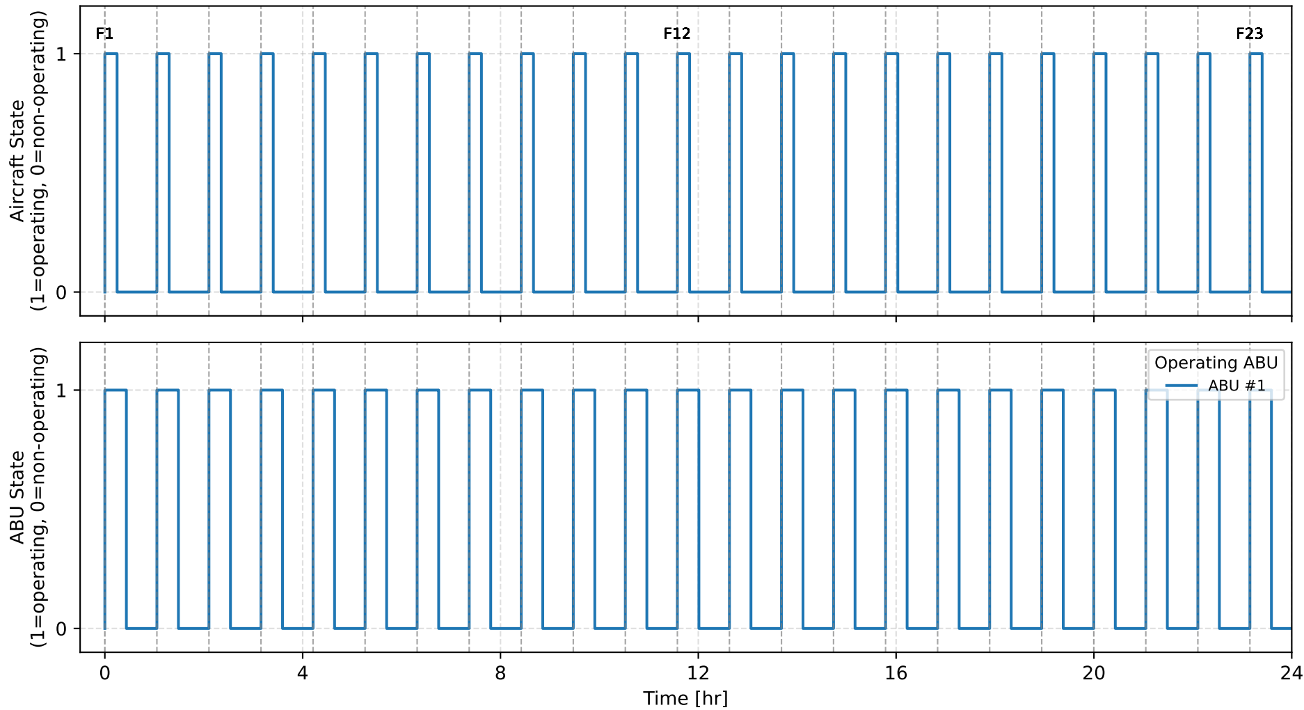
Daily Operational Timeline Number of ABUs: 1, ABU mission-energy: 5.0 kWh/ABU
