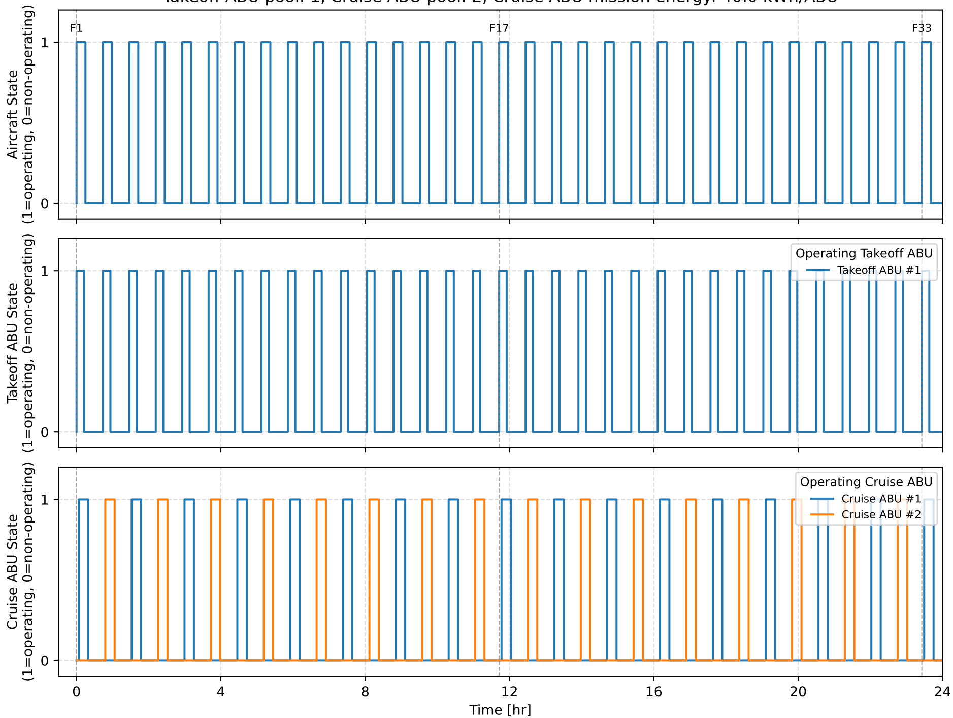
Daily Operational Timeline Takeoff ABU pool: 1, Cruise ABU pool: 2, Cruise ABU mission energy: 40.0 kWh/ABU
