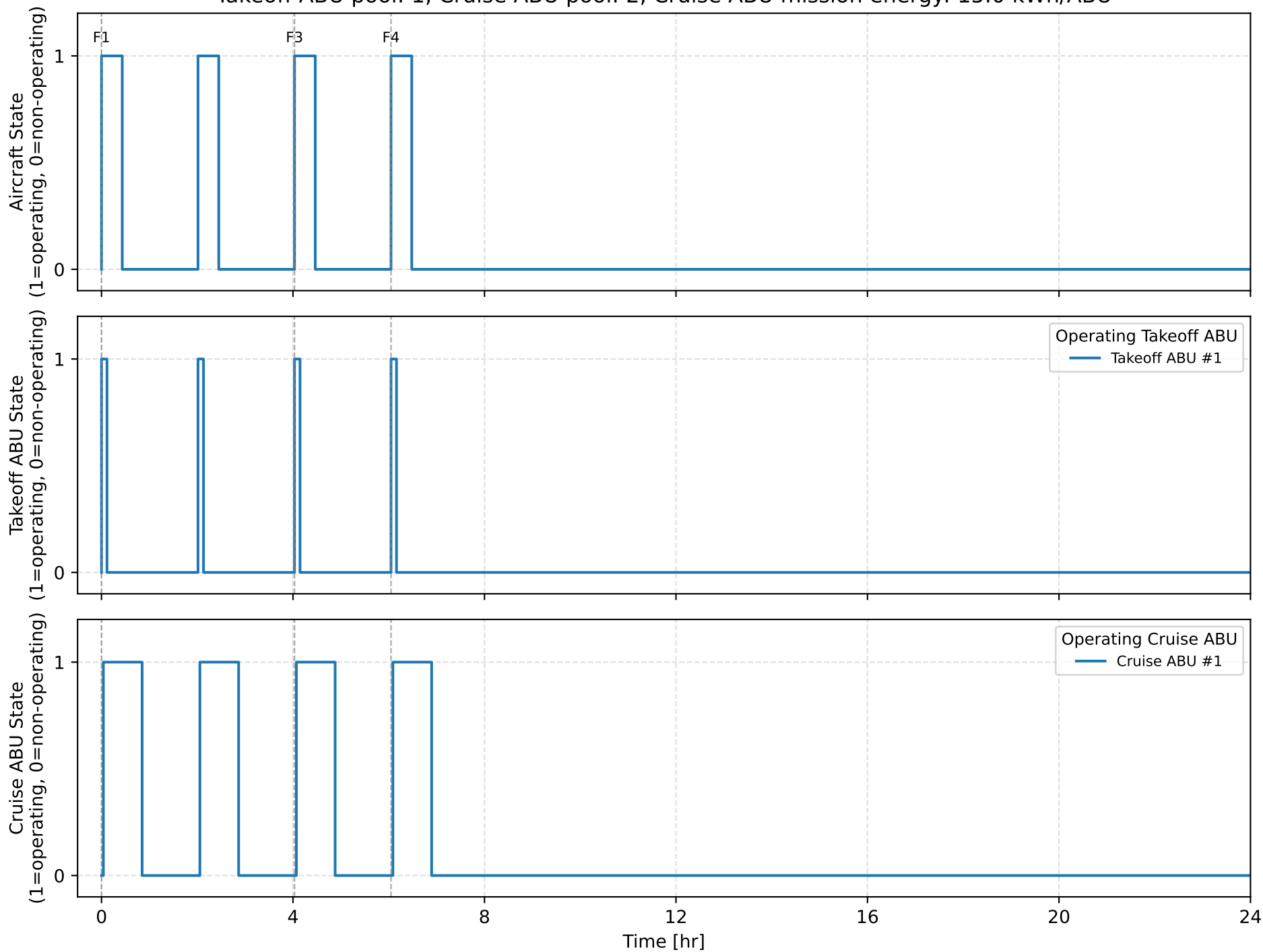
Daily Operational Timeline Takeoff ABU pool: 1, Cruise ABU pool: 2, Cruise ABU mission energy: 15.0 kWh/ABU
