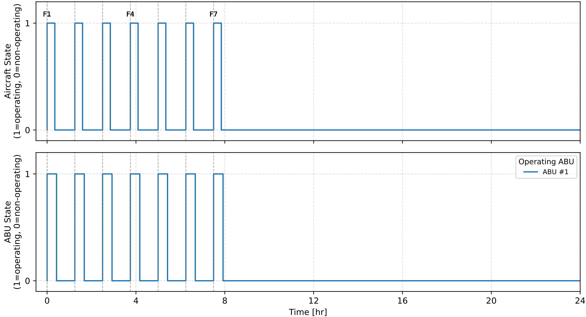
Daily Operational Timeline Number of ABUs: 1, ABU mission-energy: 50.0 kWh/ABU
