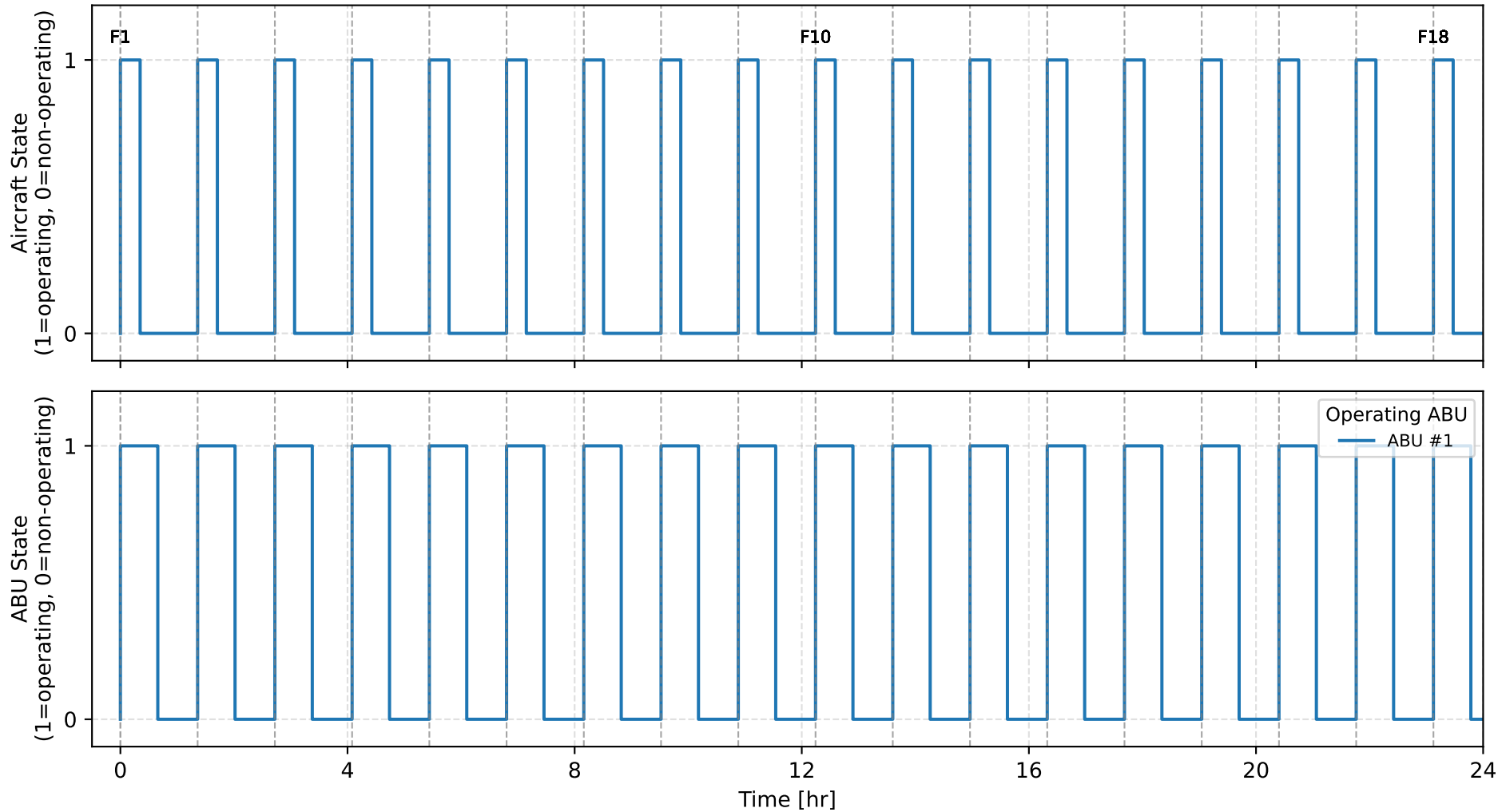
Daily Operational Timeline Number of ABUs: 2, ABU mission-energy: 5.0 kWh/ABU
