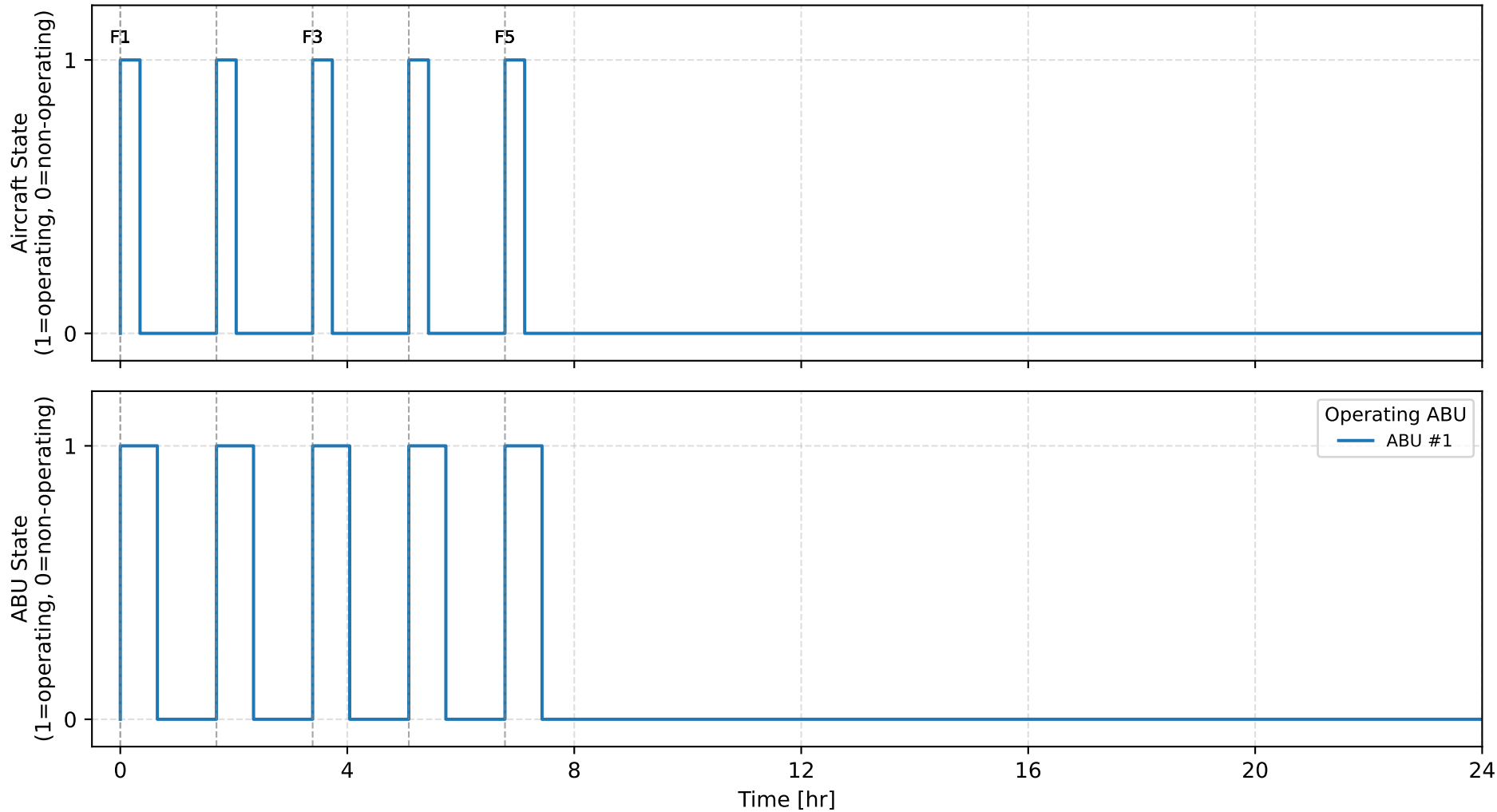
Daily Operational Timeline Number of ABUs: 1, ABU mission-energy: 10.0 kWh/ABU
