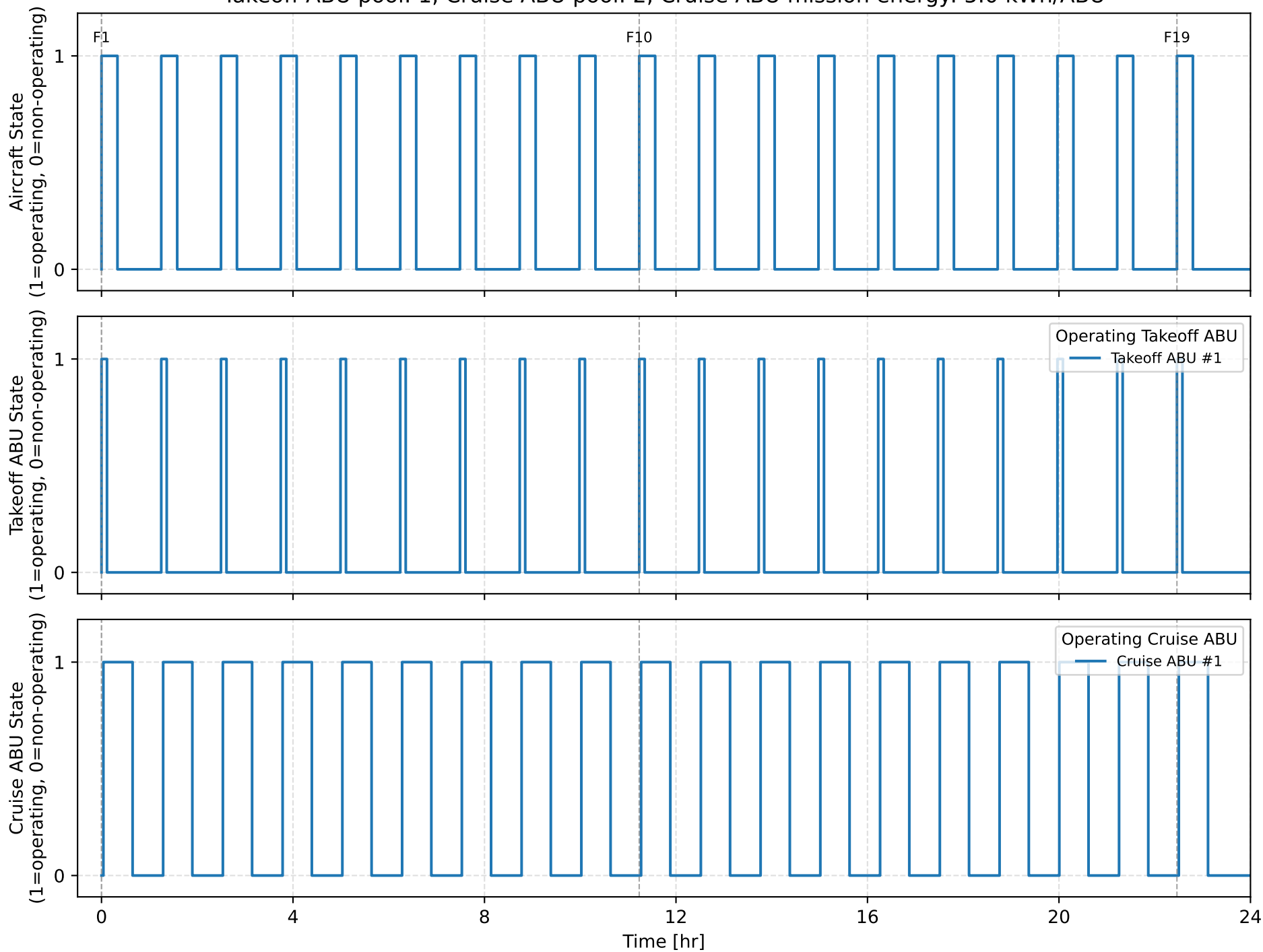
Daily Operational Timeline Takeoff ABU pool: 1, Cruise ABU pool: 2, Cruise ABU mission energy: 5.0 kWh/ABU
