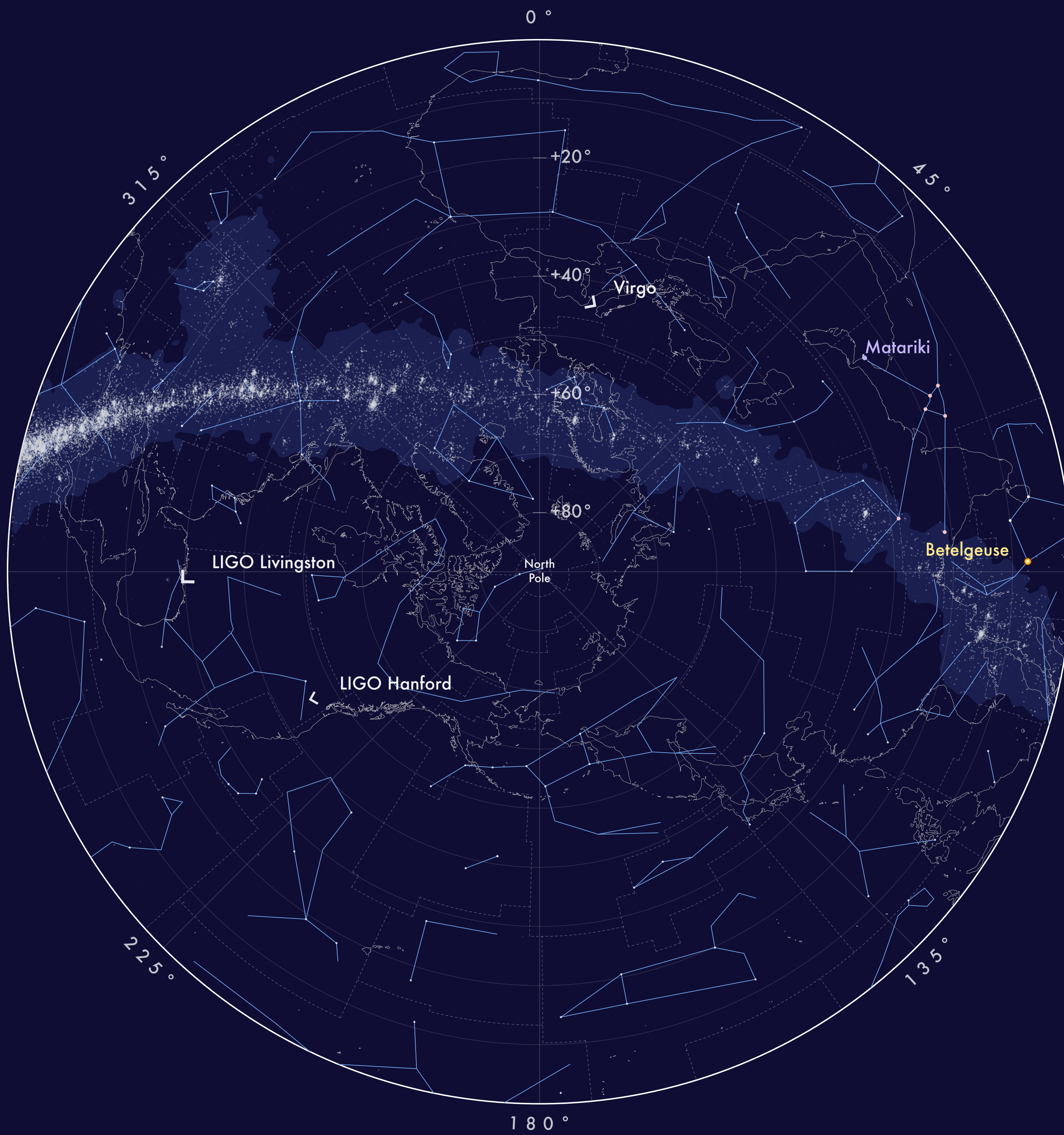
Northern Sky
