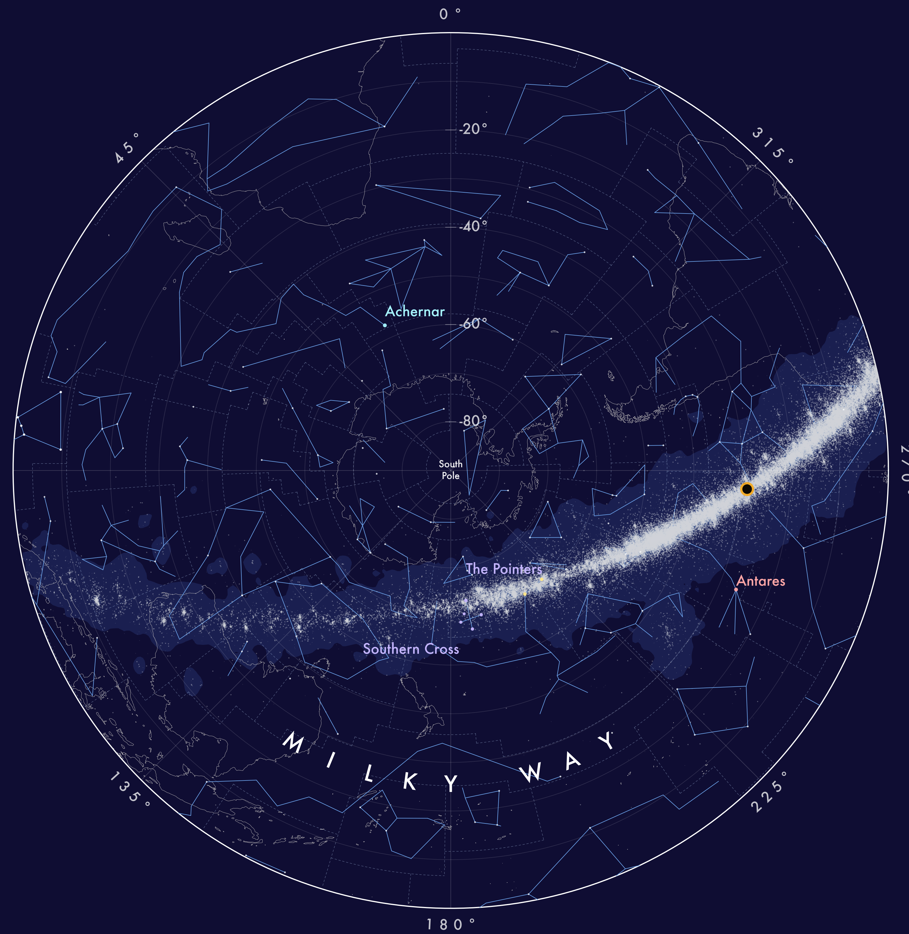
Southern Sky
