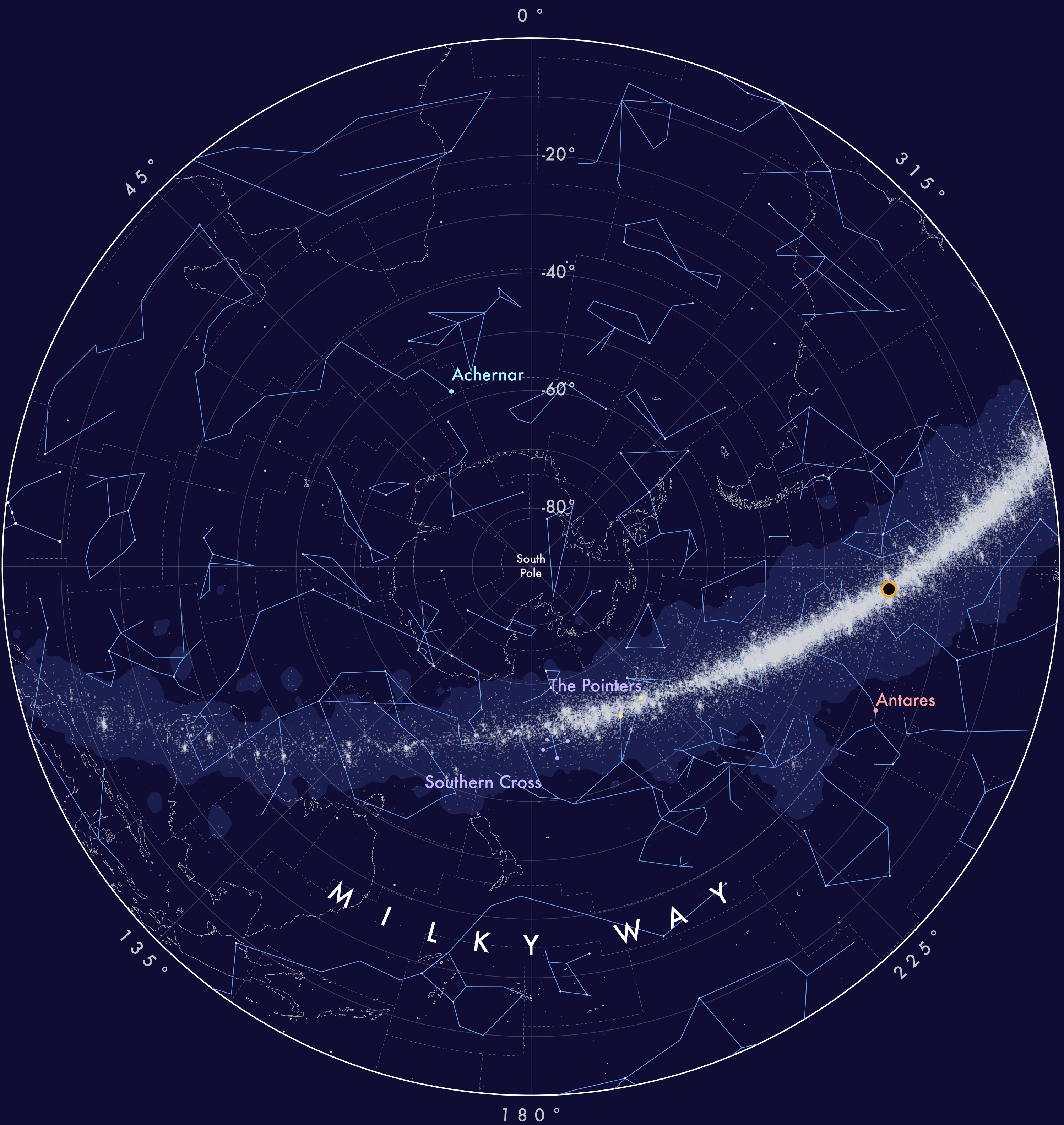
Southern Sky
