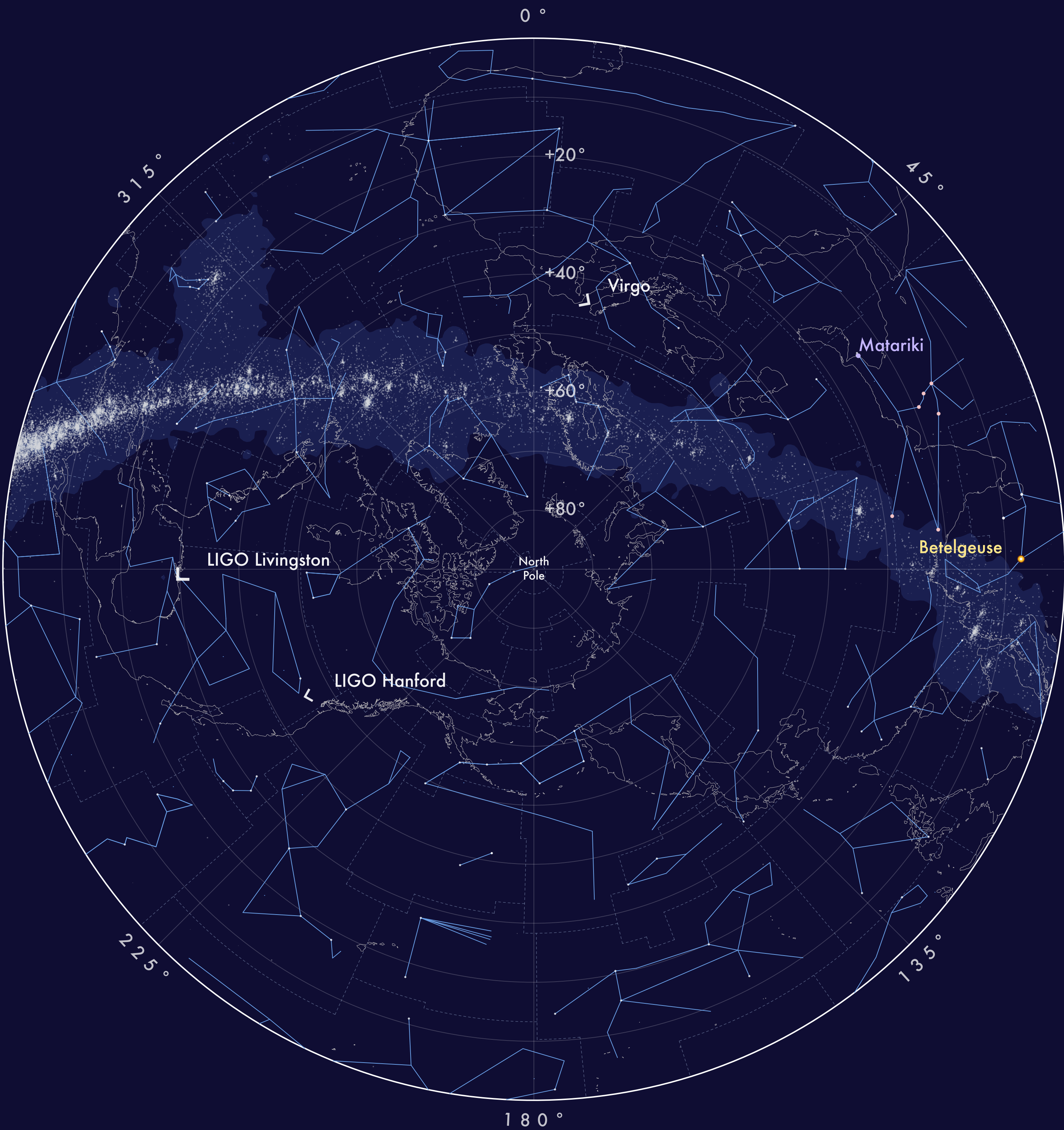
Northern Sky
