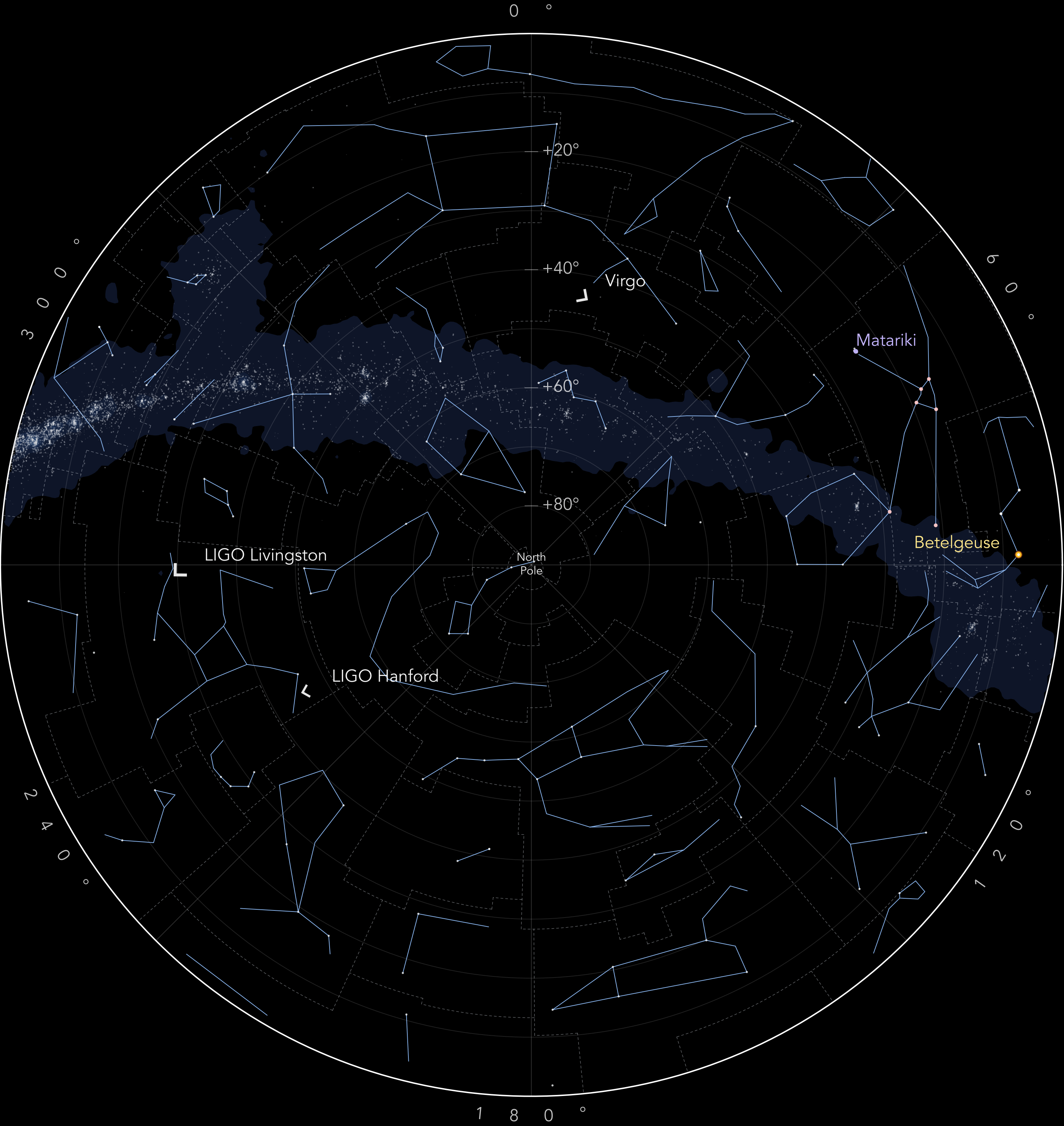
Northern Sky
