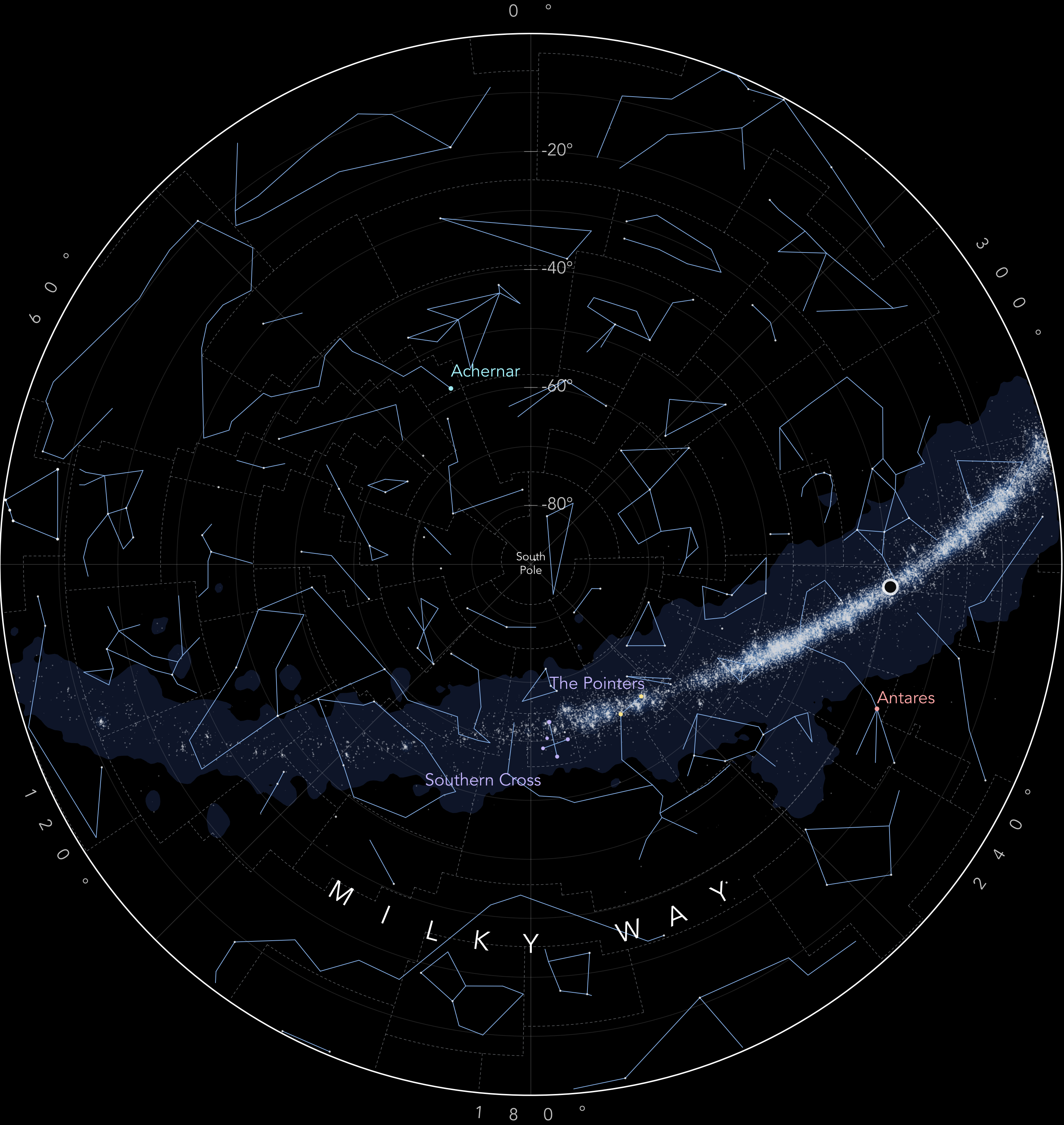
Southern Sky
