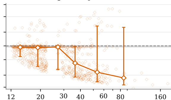
(b) L1: catalogued blips
