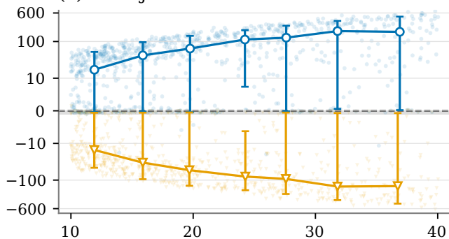
(c) H1-L1: injections
