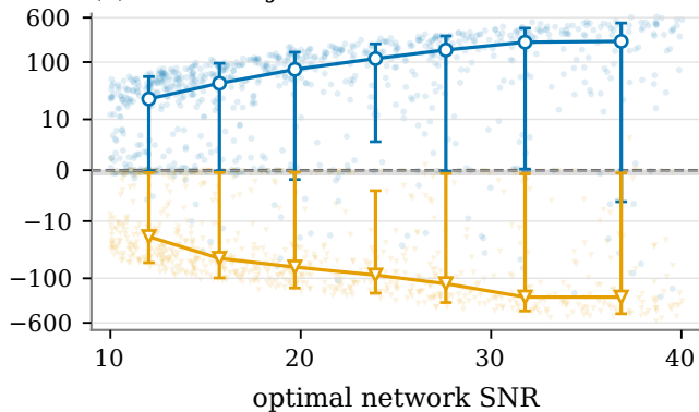
(c) H1-L1: injections
