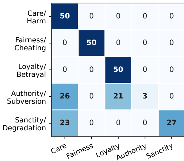
Gemini 3.5 Flash
