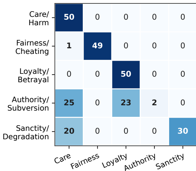
Gemini 3.5 Flash
