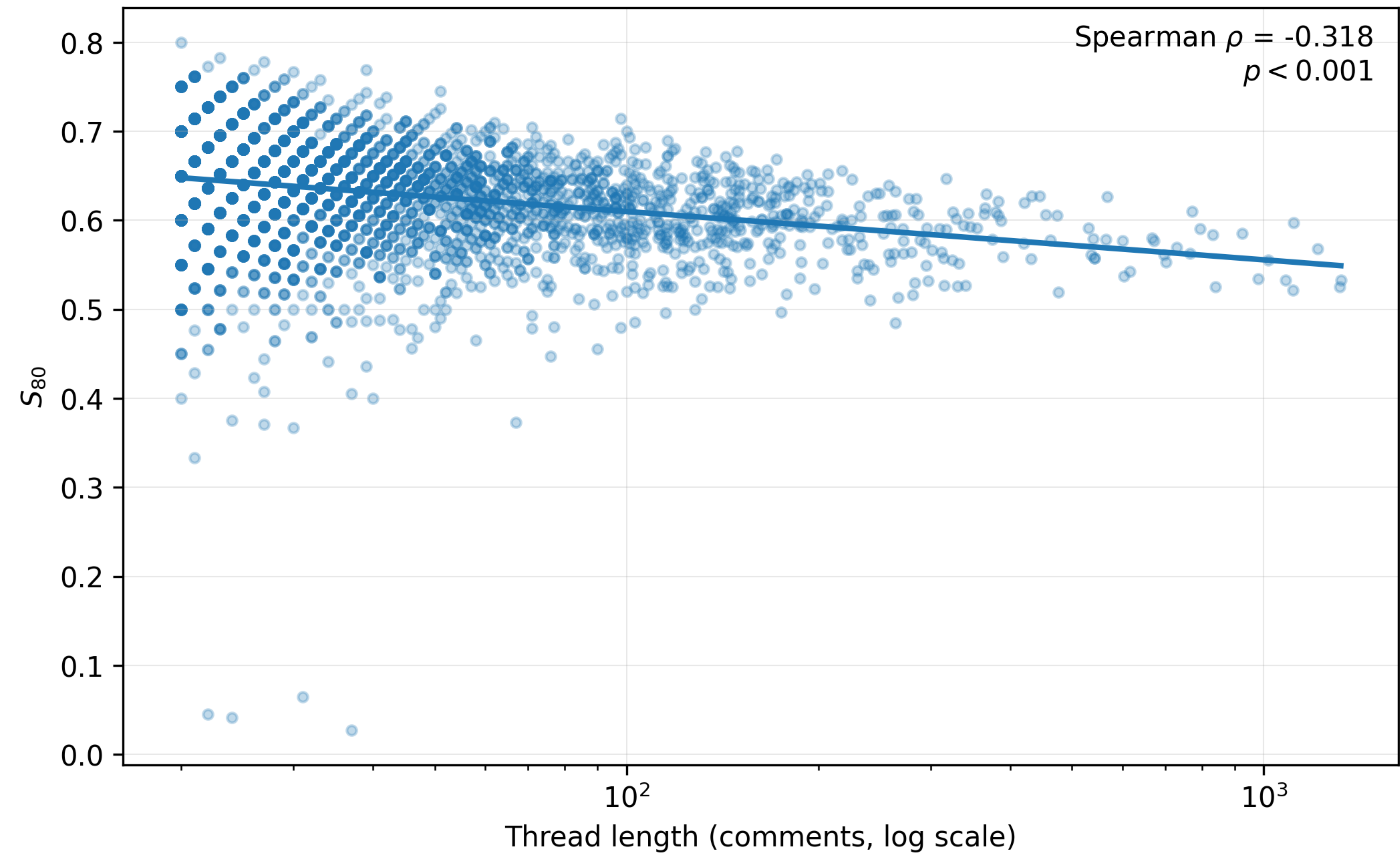
Thread Length and Semantic Saturation ( S_{80} )
