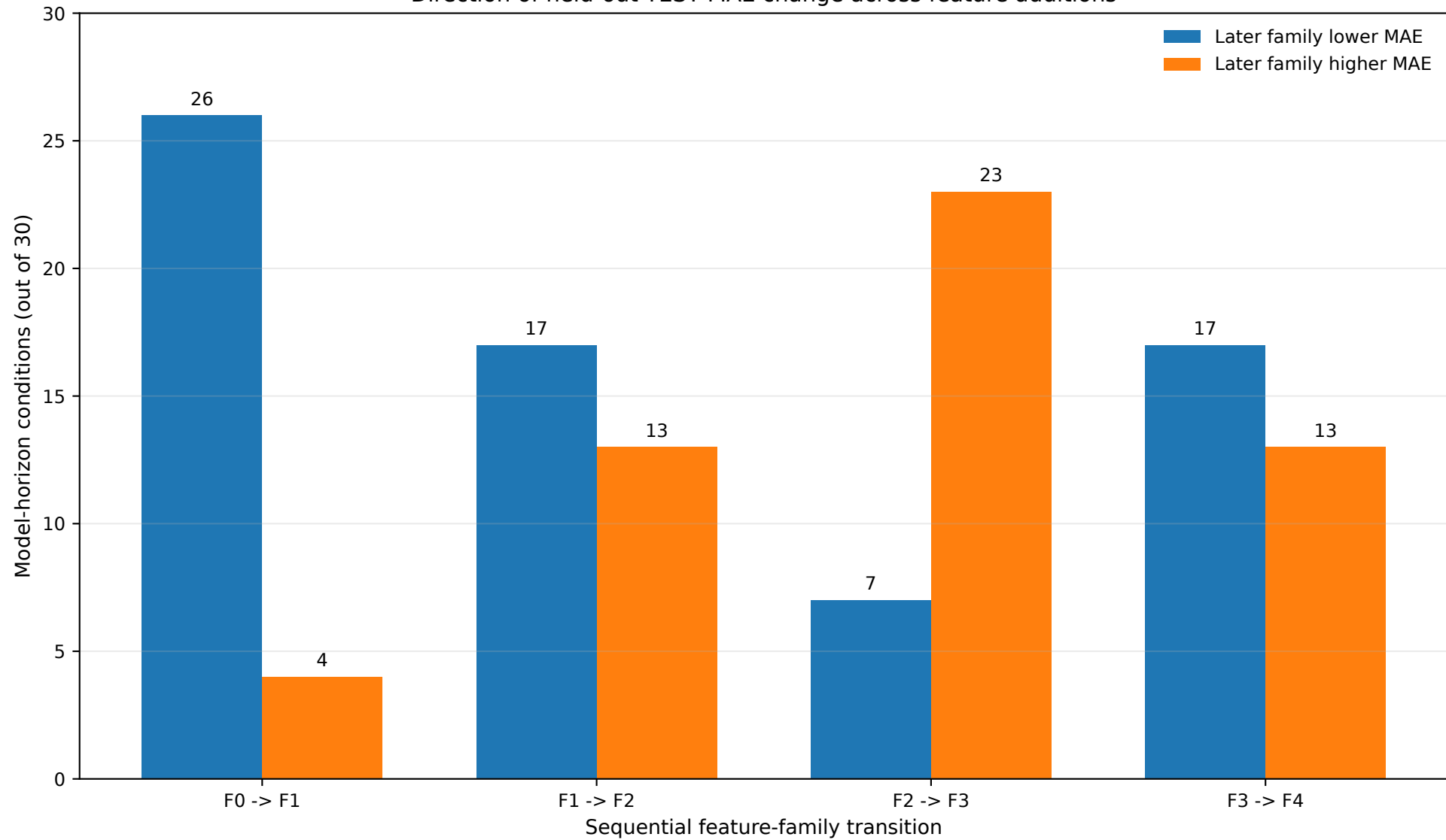
Direction of held-out TEST MAE change across feature additions
