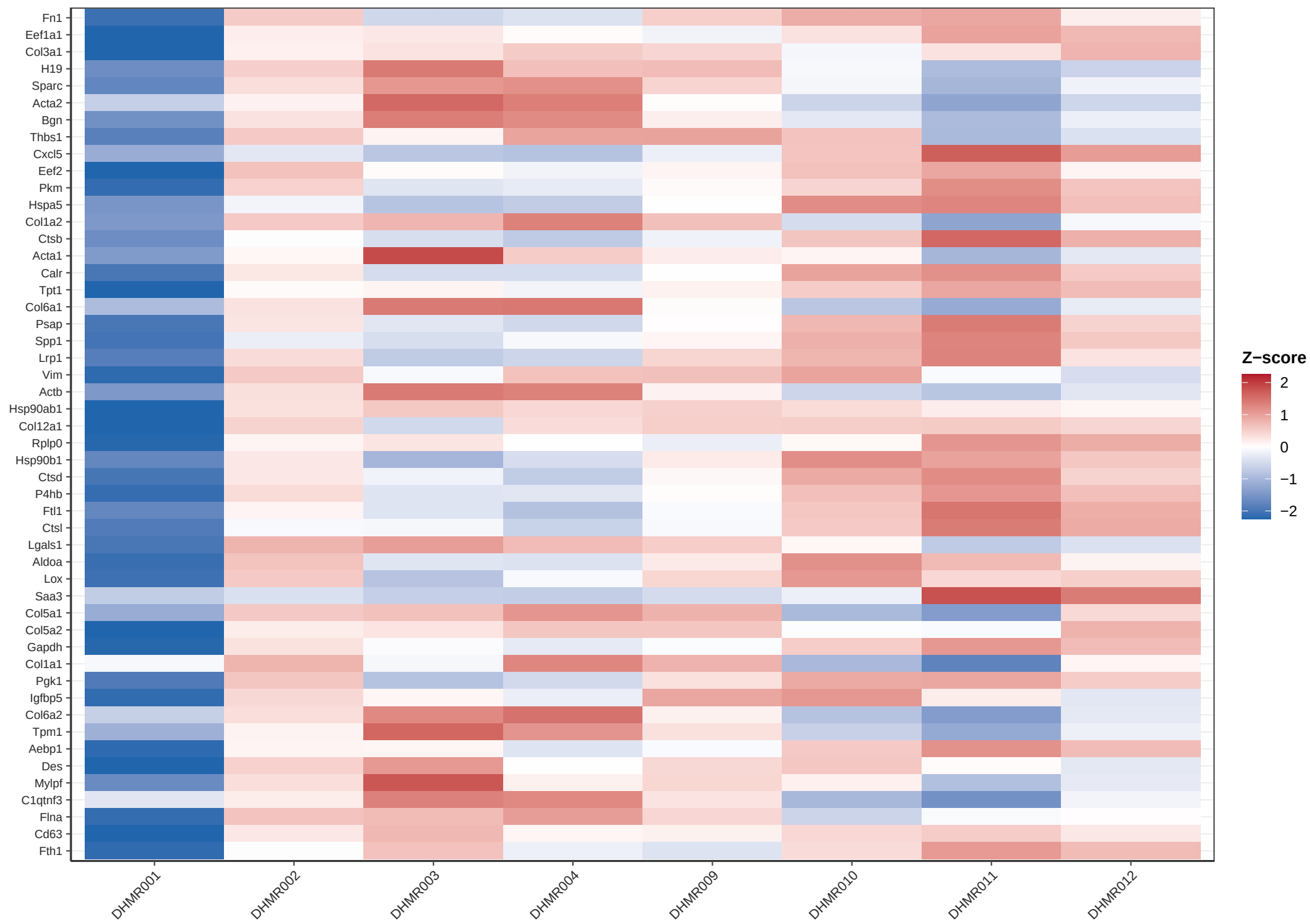
Top 50 variable features (z-scored)
