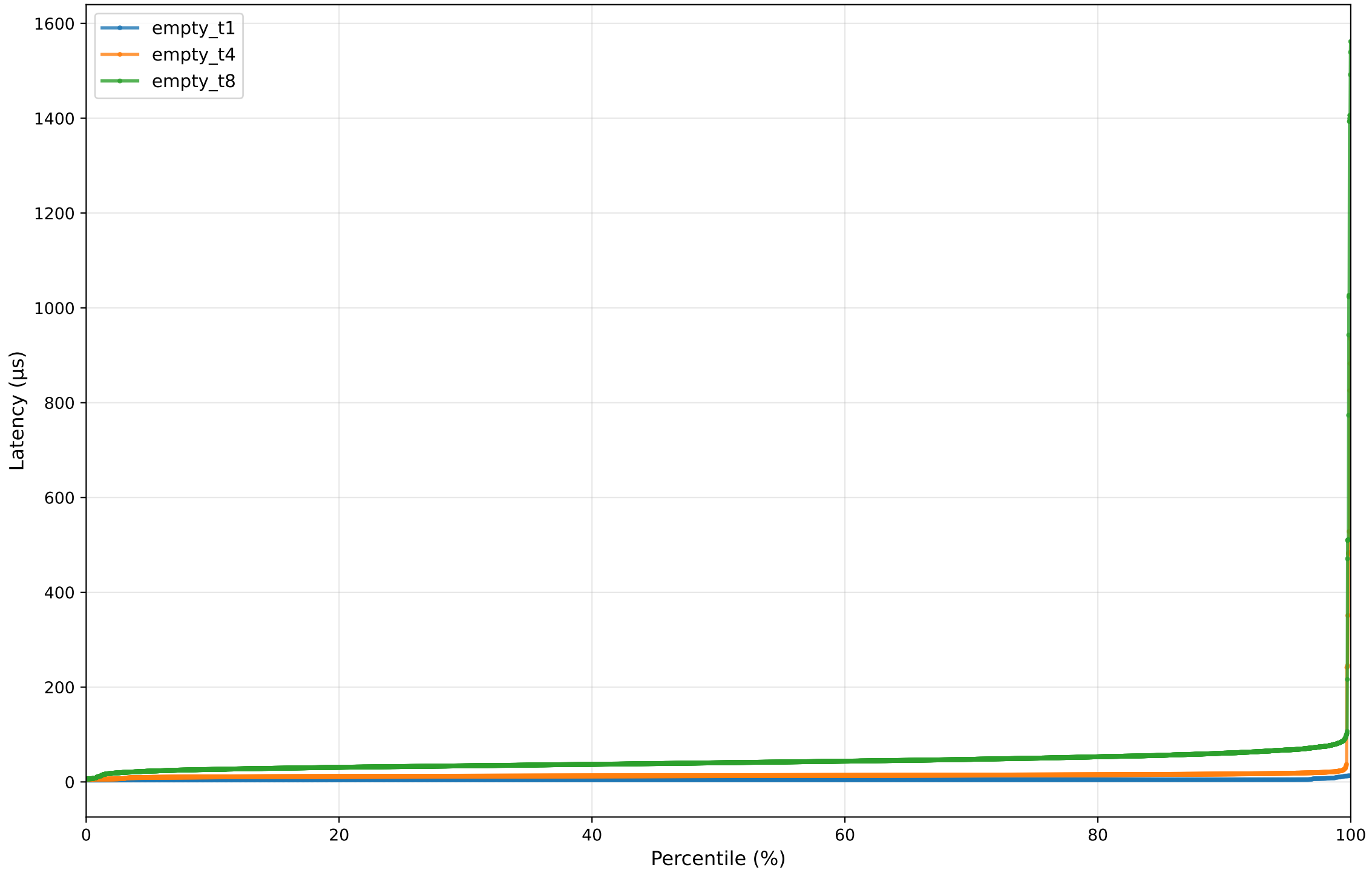
Polling Latency: Empty Queue (no FS I/O)
