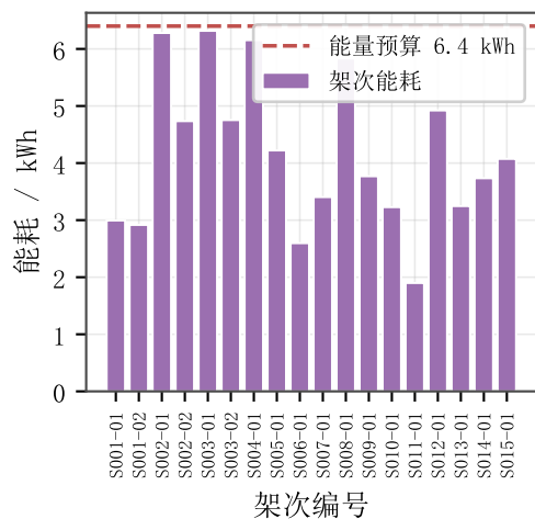
(c) 逐架次能耗均在预算内
