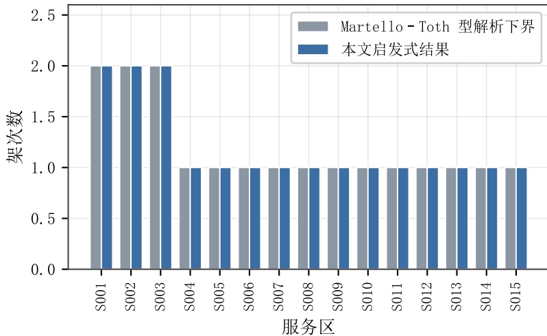
(a) 逐服务区：启发式解 = 解析下界
