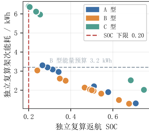
(c) 25 个架次全部满足能量约束
