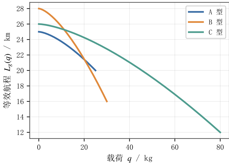
(a) 载荷—航程关系 L_g(q) = L_{g0} - (L_{g0} - L_{gF})(q/Q_g)^{3/2}
