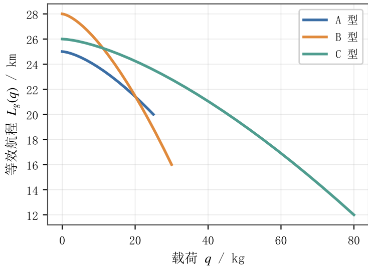
(a) 载荷—航程关系 L_g(q) = L_{g0} - (L_{g0} - L_{gF})(q/Q_g)^{3/2}
