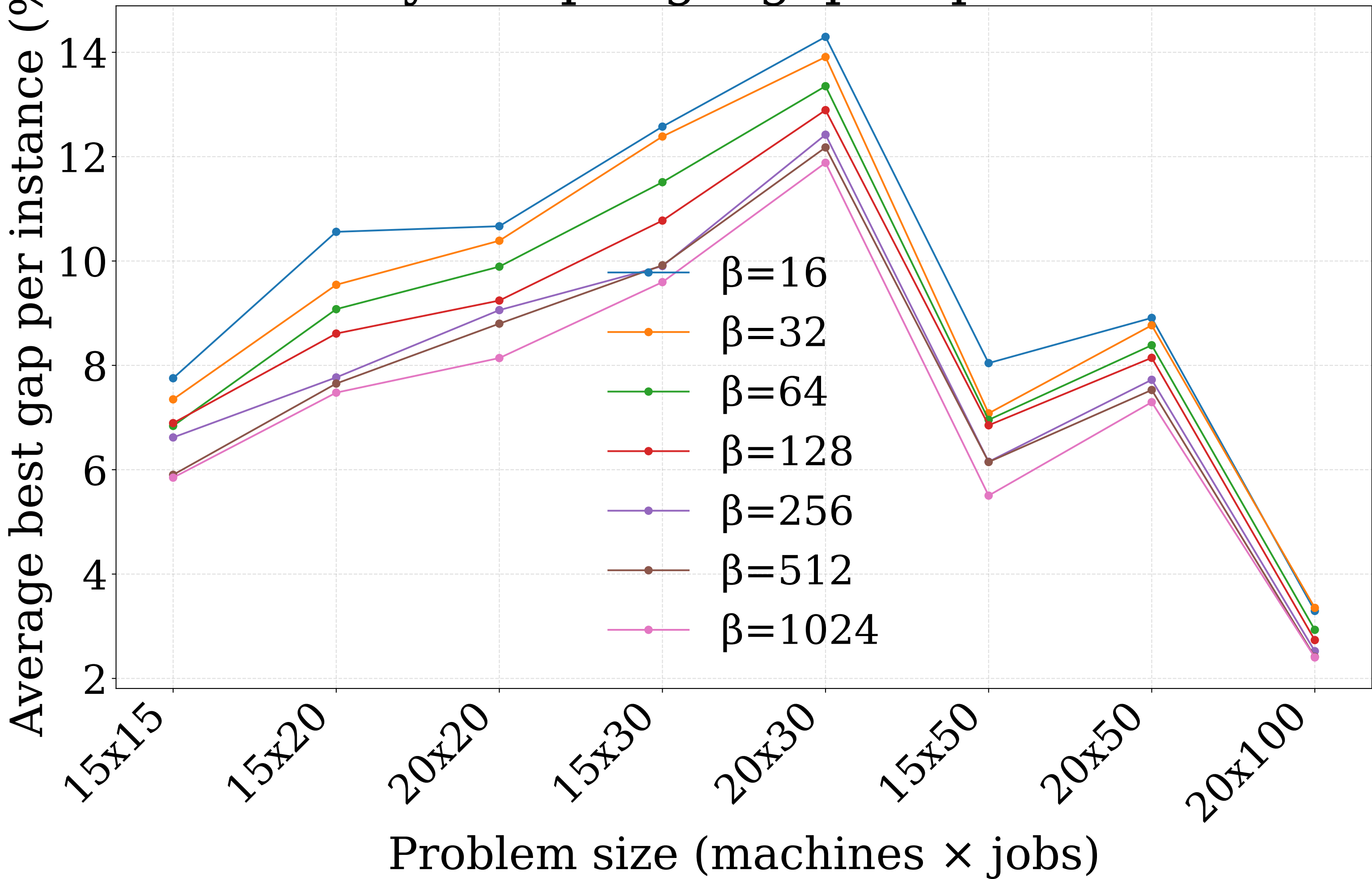
Ordinary sampling - gap vs problem size
