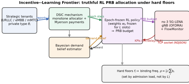
Fig. 1. GTMD-RL architecture and its 5G-LENA instantiation. Tenants submit demand reports; the RIC runs a Bayesian demand belief and an epoch-frozen RL policy that emits per-slice weights; a monotone weighted-greedy inner allocator turns weights into a PRB budget with Myerson payments. The budget is shipped over a TCP socket to the ns-3 5G-LENA gNB, which enforces it, runs the epoch on a 3GPP-compliant PHY/MAC, and returns per-slice throughput/delay as the RL reward.
