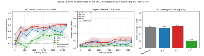
Fig. 4. Tabular contextual bandit vs. deep controllers (DQN/PPO/A2C) on the same 28-action simplex and priced-mechanism reward. (a) normalized reward and (b) optimal-action rate vs. training epoch (mean \pm std, 3 seeds); (c) converged normalized reward. \text{PPO} \geq \text{tabular} \approx \text{DQN} \gg \text{A2C} .
