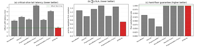
Fig. 6. Per-slice view at overload ( \eta=1.3 ). The aggregate p95 is dominated by the delay-tolerant mMTC slice (20 ms budget) and hides what matters: the deployed GTMD-RL scheduler—deadline- and channel-aware, with a small proactive burst headroom for the tight-SLA slice—delivers the lowest URLLC tail latency (a), the best priority-weighted SLA (b), and, uniquely among demand-aware policies, guarantees hard floors (c).
