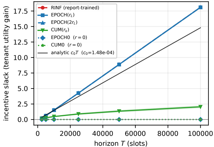
(a) fragility, the gate, and exact invariance
