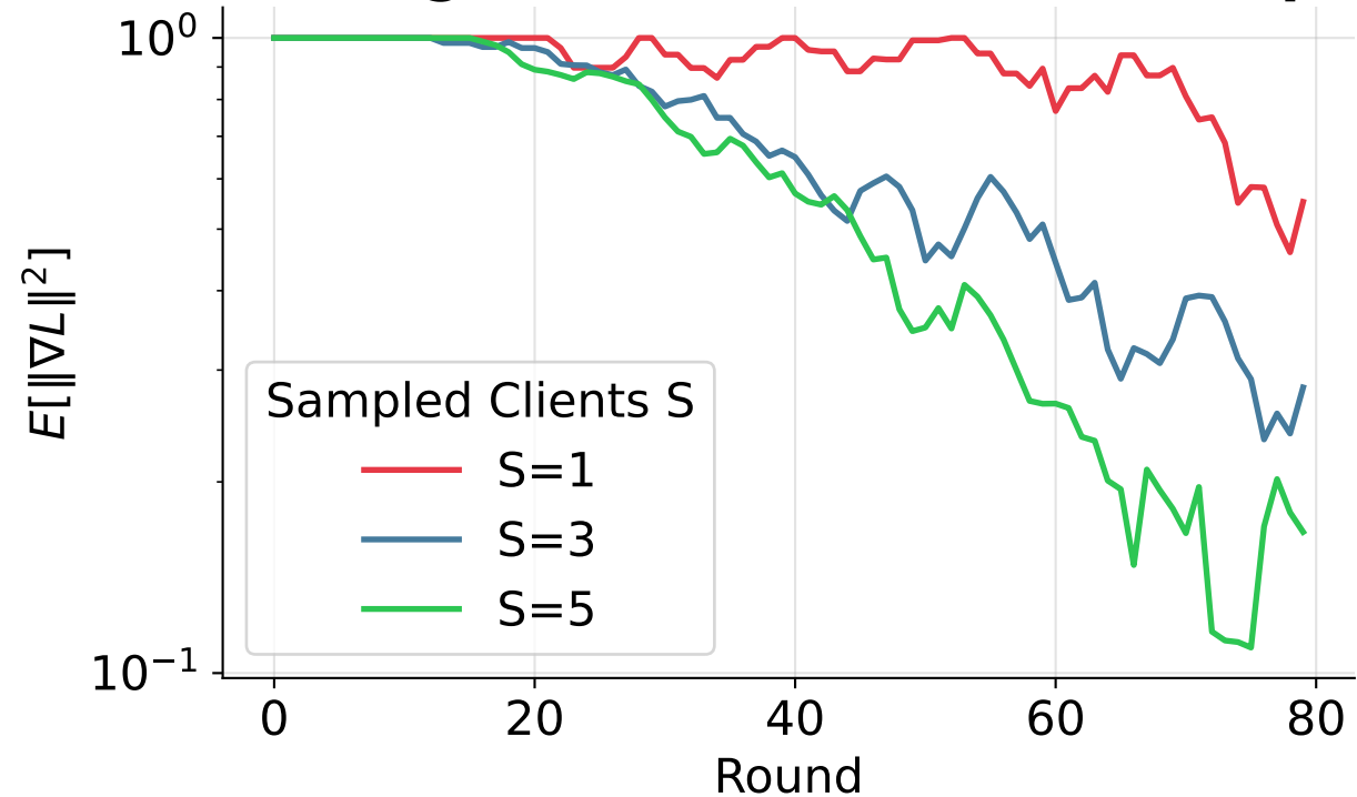
(a) Convergence under Partial Participation
