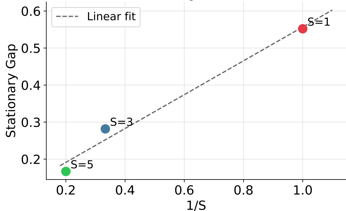
(b) Gap vs 1/S
