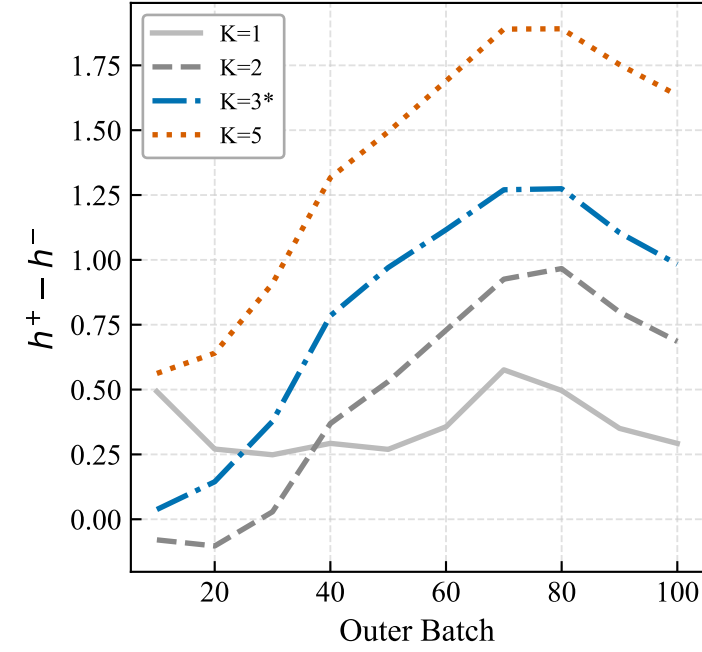
Train Reward Margin
