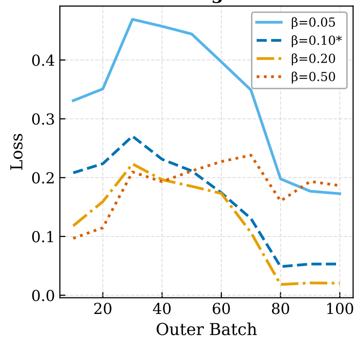
Training Loss
