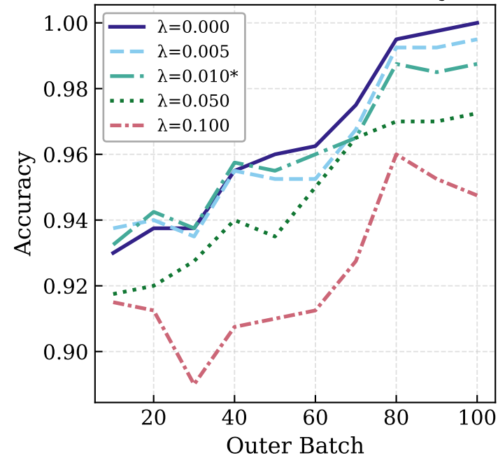
Train Reward Accuracy
