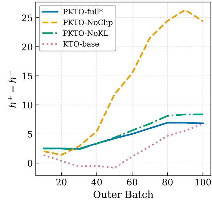
Train Reward Margin
