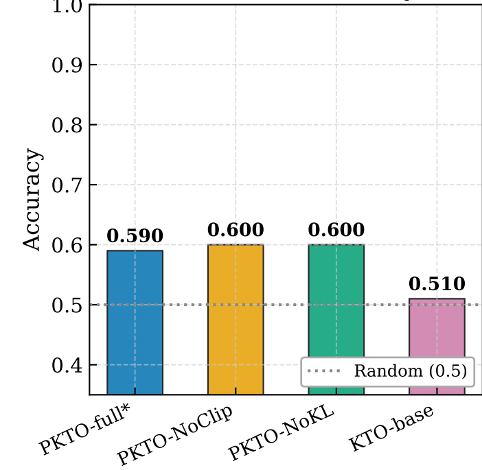
Final Eval Accuracy
