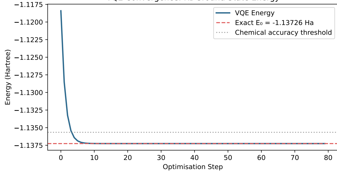
VQE Convergence: H 2 Ground State Energy
