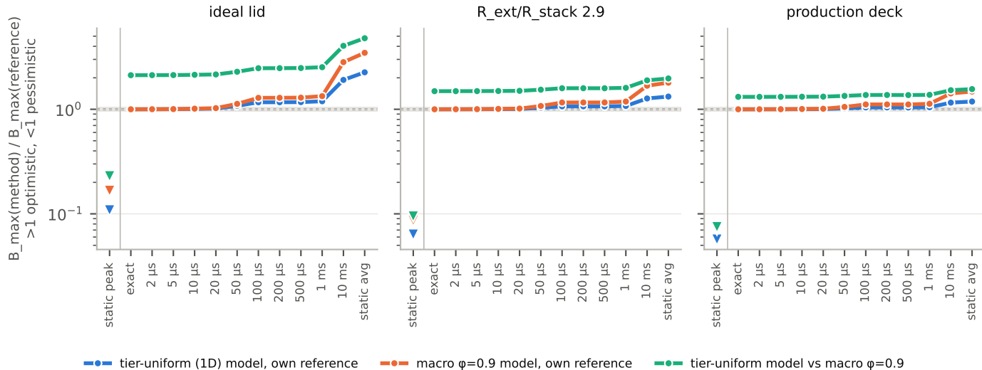
Temporal input vs reference, schedule: S1 on the measured kernel trace; shaded \pm 5\%
