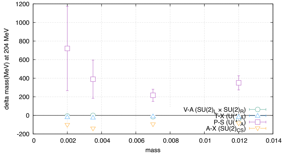
Symmetry Mass Differences at T=204 MeV
