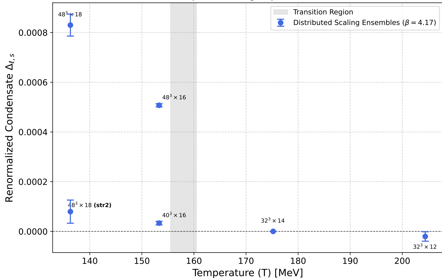
Finite Volume & Temporal Scaling at \beta = 4.17 (Distributed Runs)
