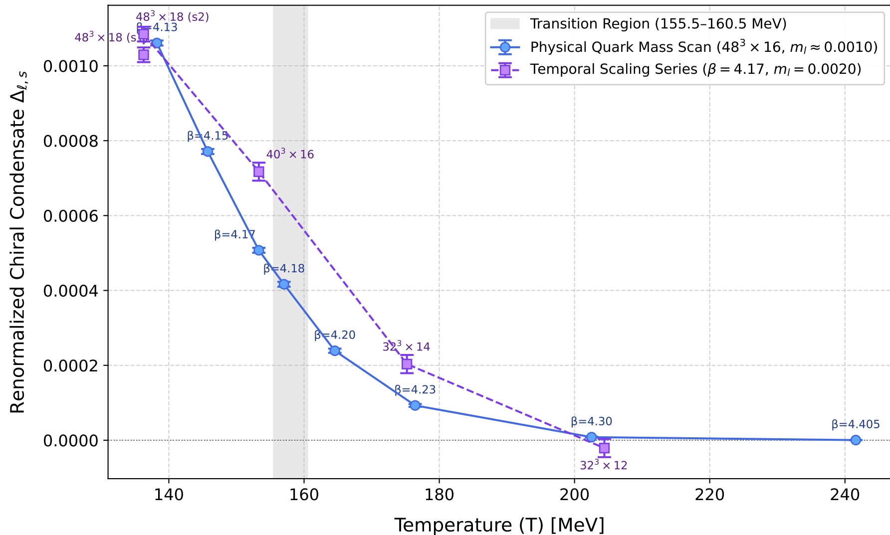
Global Chiral Condensate \Delta_{\ell,s} vs Temperature (All 13 Ensembles)
