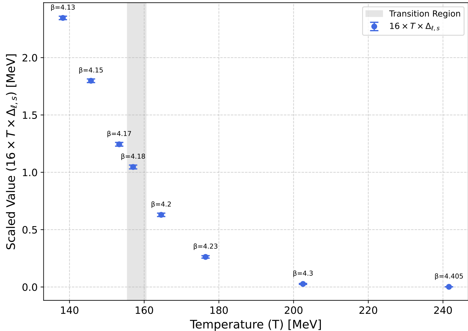
Scaled \bar{\psi}\psi vs Temperature (ana Standard)
