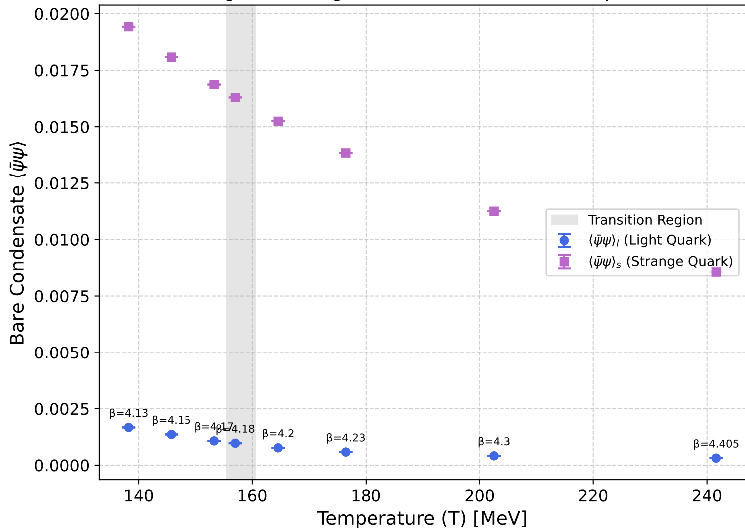
Bare Light & Strange Quark Condensate vs Temperature
