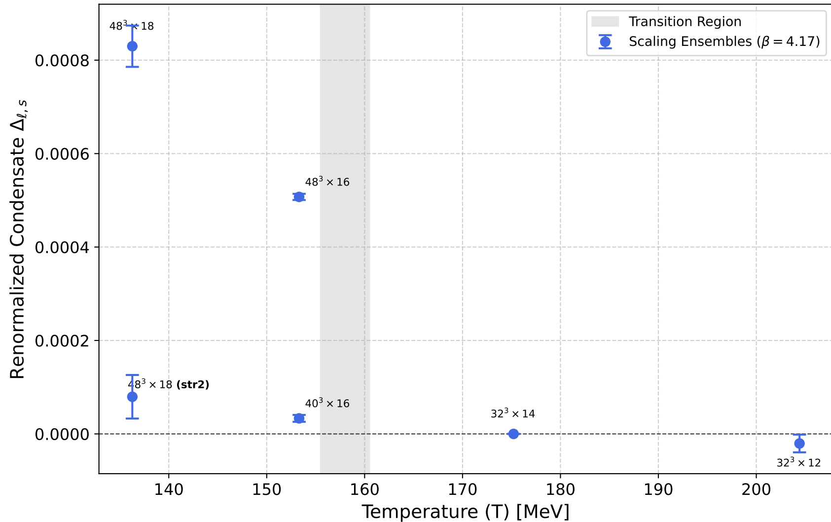
Finite Temporal Scaling Condensate at \beta = 4.17
