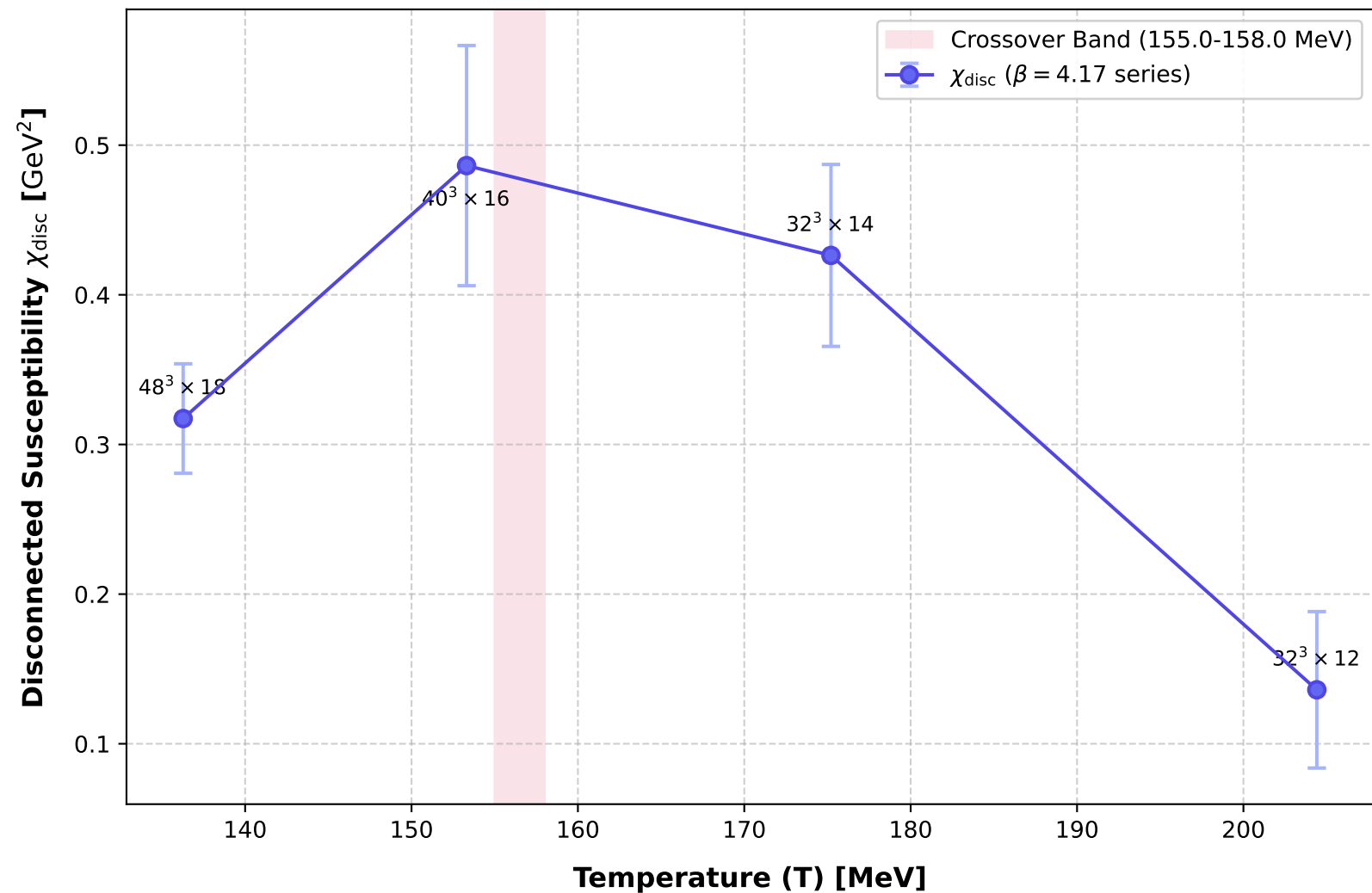
Disconnected Chiral Susceptibility vs Temperature ( \beta = 4.17 )
