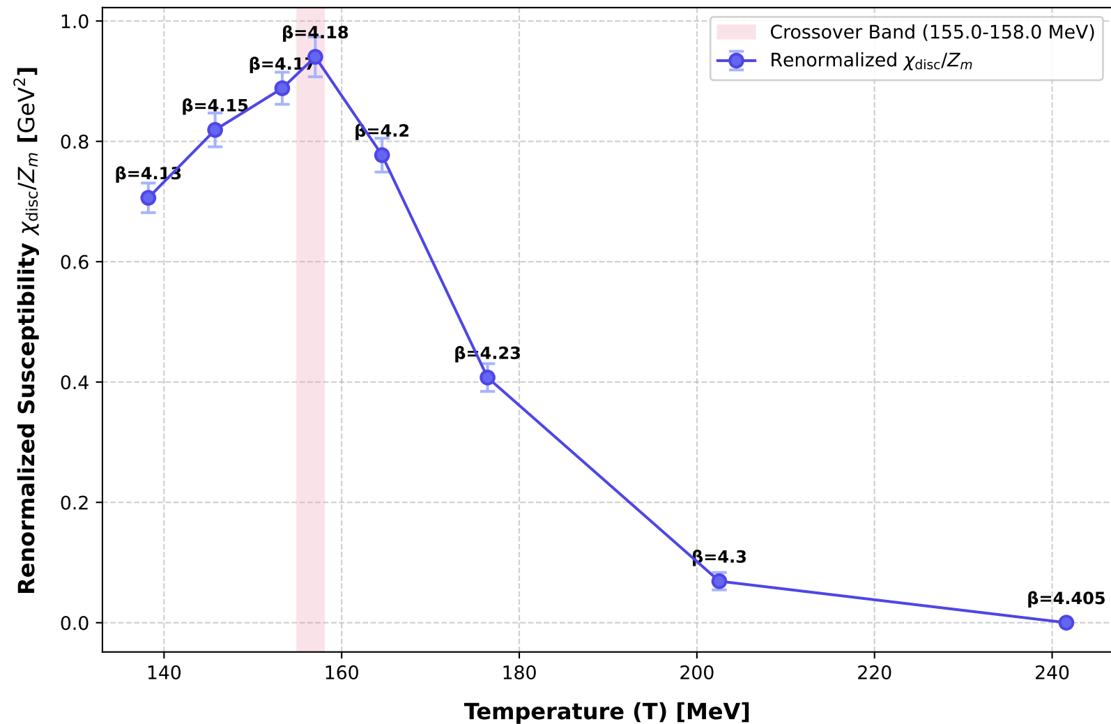
Renormalized Chiral Susceptibility \chi_{\text{disc}}/Z_m vs Temperature
