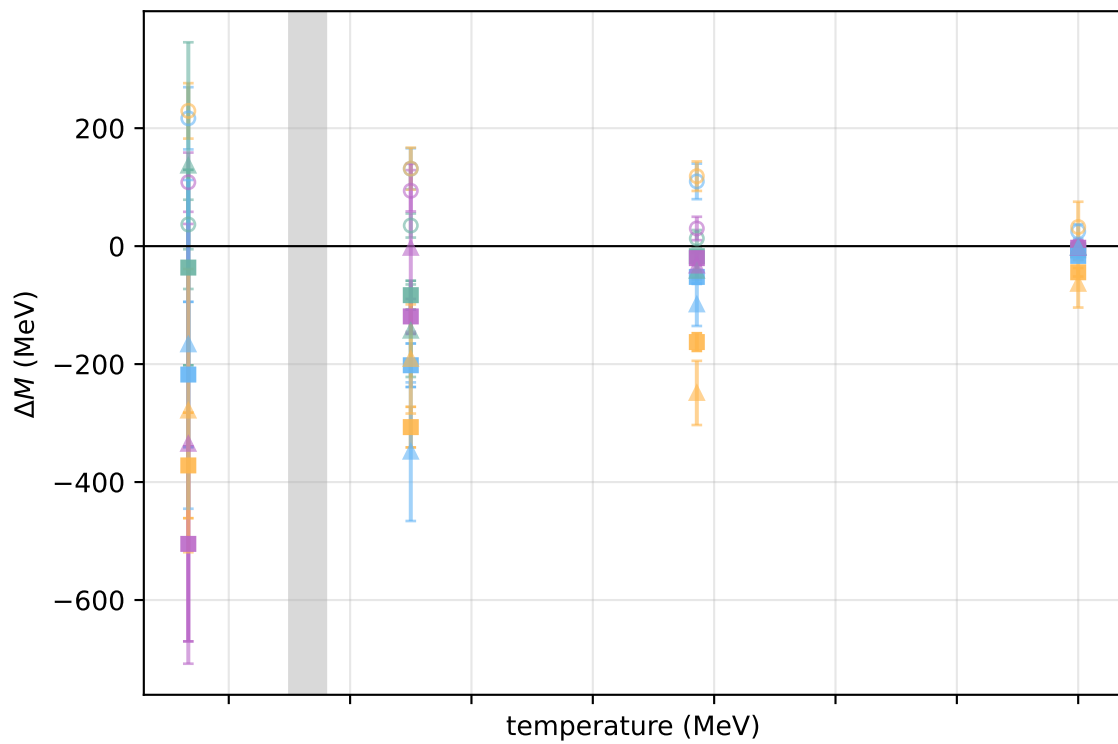
U(1) S-PS
