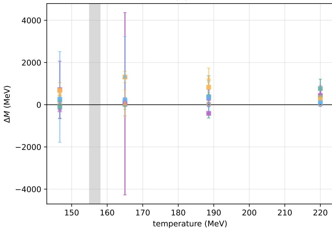
U(1) S-PS
