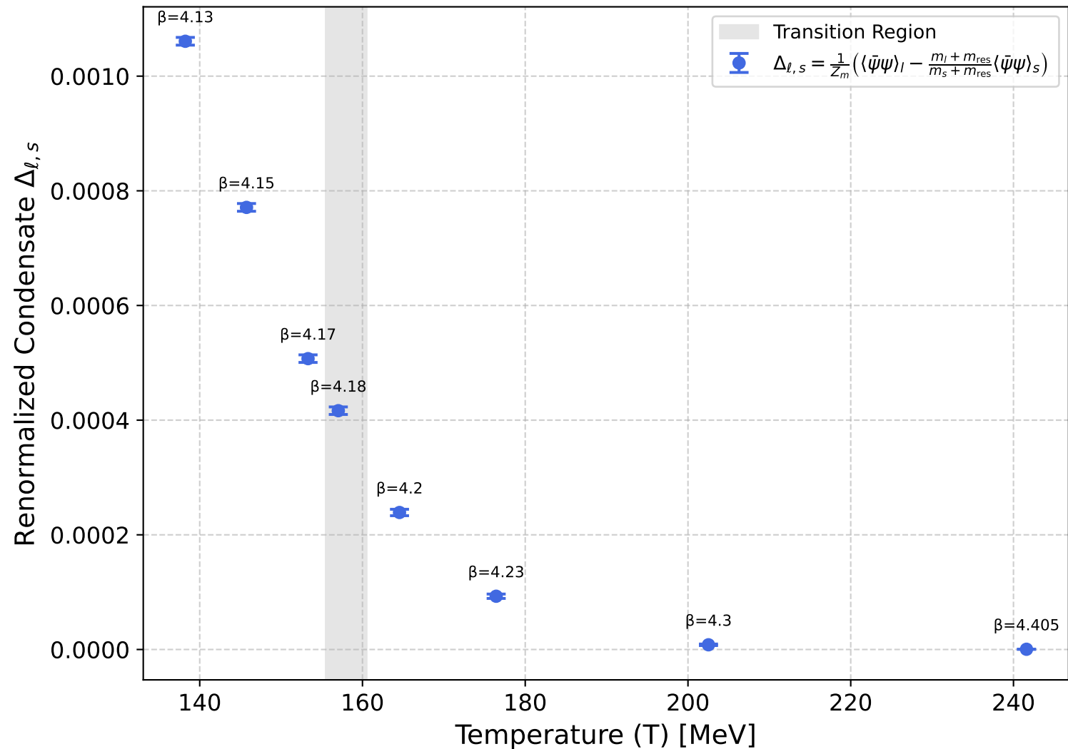
Renormalized \bar{\psi}\psi vs Temperature ( 48^3 \times 16 Series)
