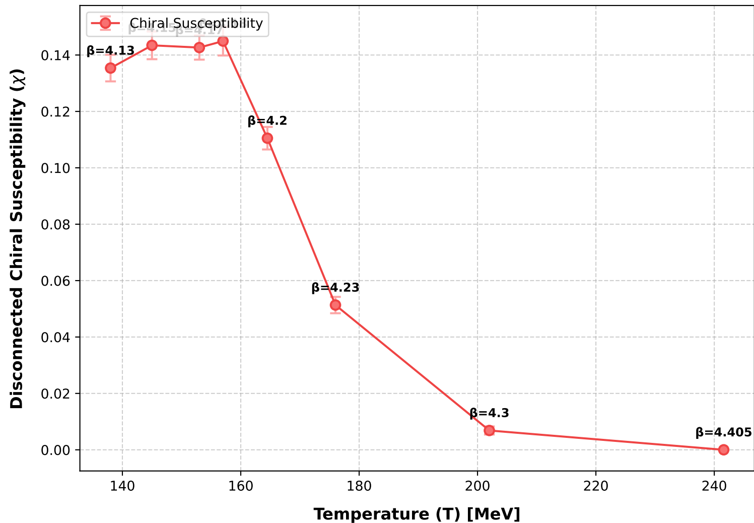
Disconnected Chiral Susceptibility \chi vs Temperature
