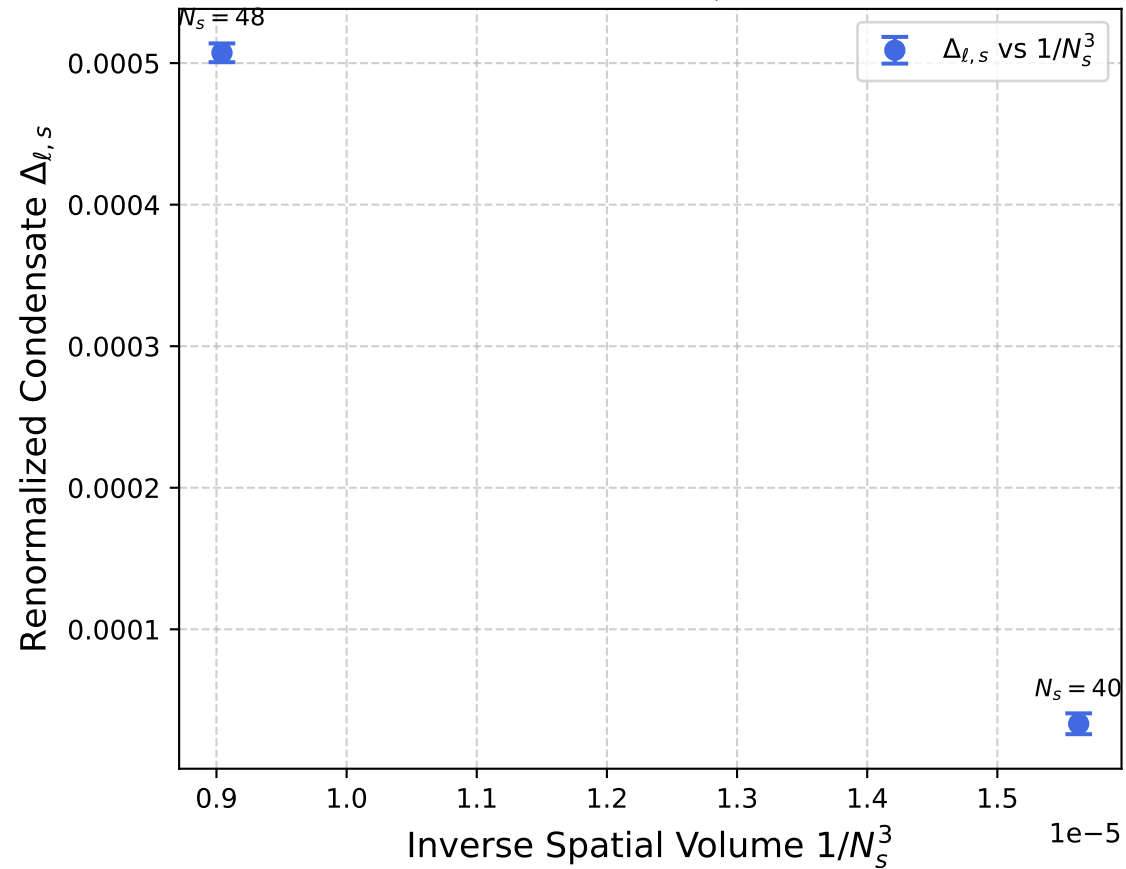
Finite Volume Scaling of \Delta_{l,s} ( T = 153.31 MeV)
